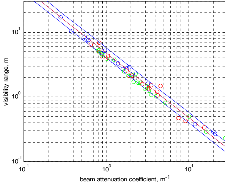
Fig. 3. Horizontal visibility of a 200 mm diameter black target. Colors of circles refer to three different observers. Red line indicates vis. range = y = 4.5/\alpha and the blue lines are \pm 20\% lines; \alpha = \text{photopic attenuation coefficient} = 4.5 / [c_{pg}(532) * 0.9 + 0.081] ; r^2 = 0.985 . (From Zaneveld and Pegau, 2003). Diver visibility ranges are also closely related to bottom depth detection and bottom type discrimination capabilities for passive imaging systems.
