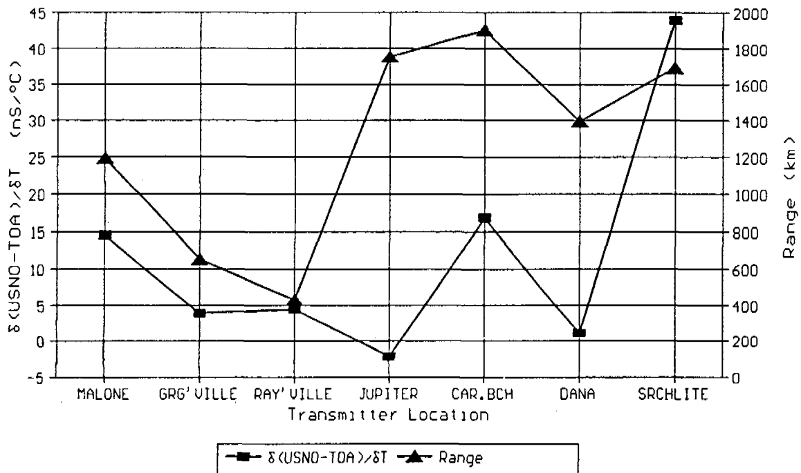
FIG. 12--Loran-C \delta(\text{USNO-TOA})/\delta T vs Range from Time/Temp. Regression
