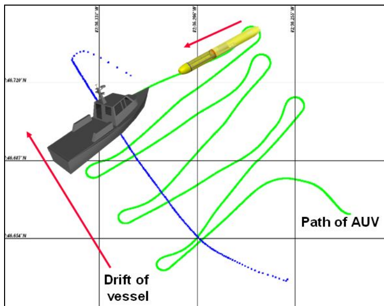
Figure 6. The ship hull scanning setup: the AUV scans the drifting target vessel.
