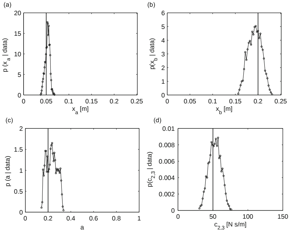
Fig. 5. Calculated posterior distributions of, respectively, (a–d) delamination start point x_a , delamination end point x_b , delamination depth a , and local damping coefficient c_{2,3} .
