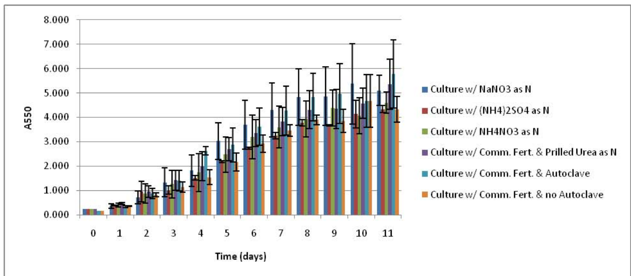
Figure 4.12 and Figure 4.13: Results from Experiment 5. Figure 4.12 reflects changes in cell concentration with time, while Figure 4.13 reflects absorbance changes with each culture, and the error associated with each measurement. Note the growth exhibited by the cultures using (\text{NH}_4)_2\text{SO}_4 and \text{NH}_4\text{NO}_3 as "N" when pH is adjusted every day to \sim 6.6 .
