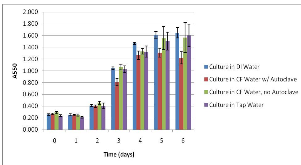
Figure 4.4 and Figure 4.5: Results from Experiment 1 depicting C. vulgaris yield through growth in BBM with 4 x NaNO 3 using different water types. Figure 4.4 reflects cell concentration changes with time while Figure 4.5 reflects A550 changes with time, and the error associated with each measurement. Note the performance of the culture grown in the media containing autoclaved Charcoal Filtered Tap Water.
