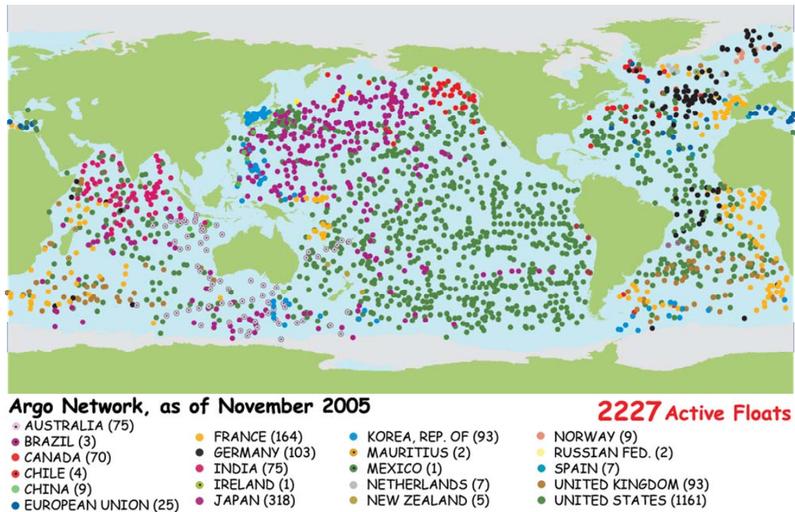
Figure 2: The Argo Array as of 30 November 2005 (US floats in Green)
