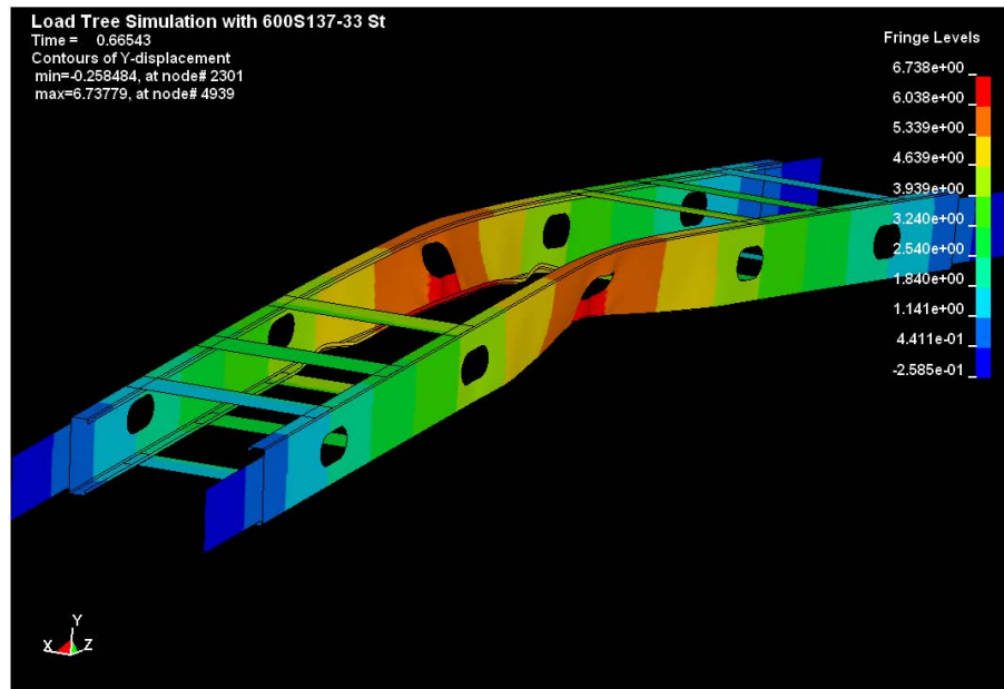
Figure 7: Simulation of Load Tree Specimen with Idealized Connections
