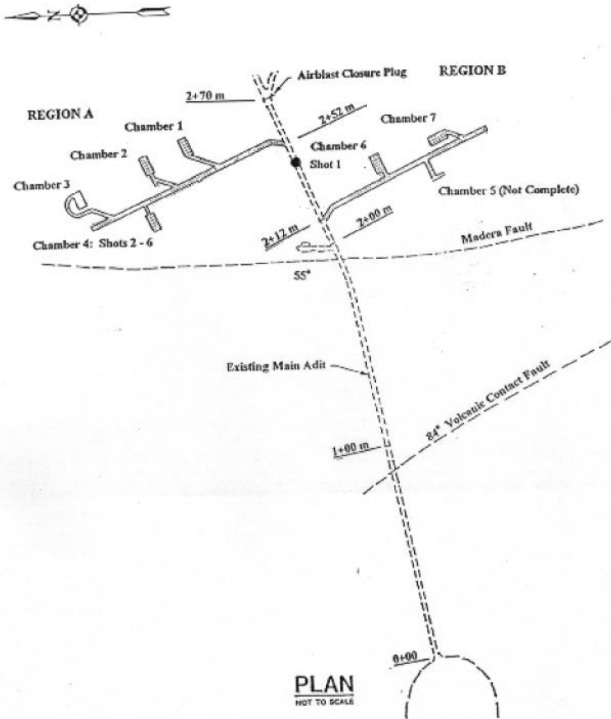
Figure 1. U.S./ROK UAST PROGRAM -- U.S. Intermediate-Scale test site layout, Tests 1 through 6 at the Lynchburg Mine near Magdalena, NM.
