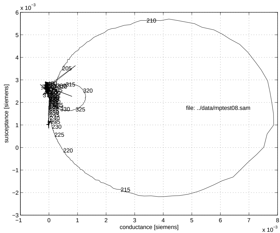
Figure 72: 2006 Lake Washington admittance loop, file MPTTEST08.DAT
