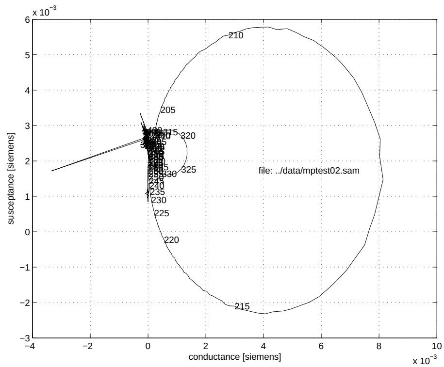
Figure 66: 2006 Lake Washington admittance loop, file MPTTEST02 . DAT
