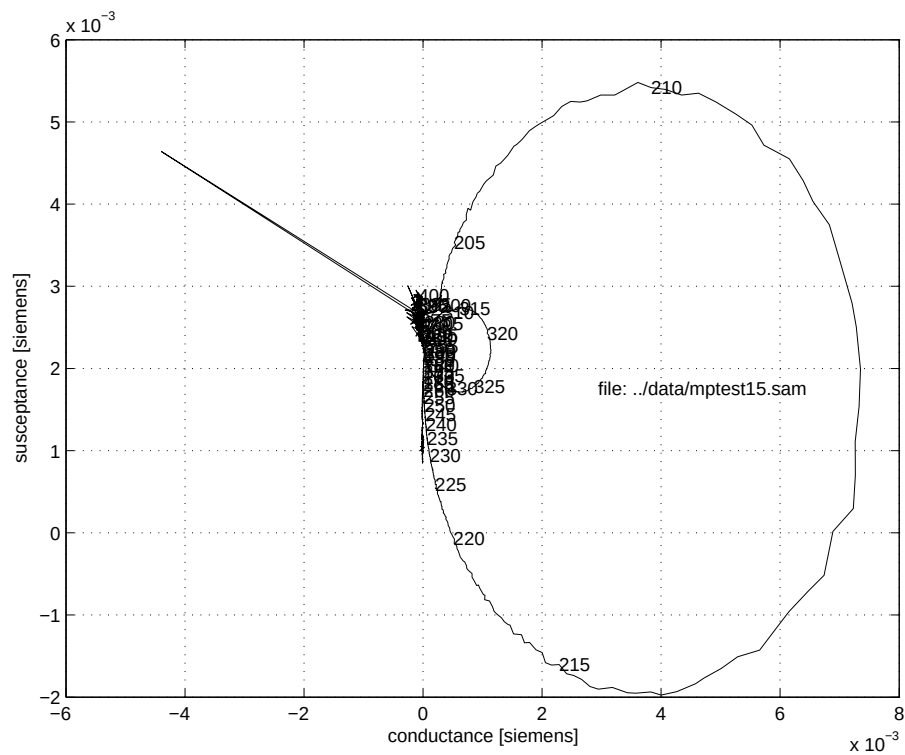
Figure 77: 2006 Lake Washington admittance loop, file MPTTEST15.DAT
