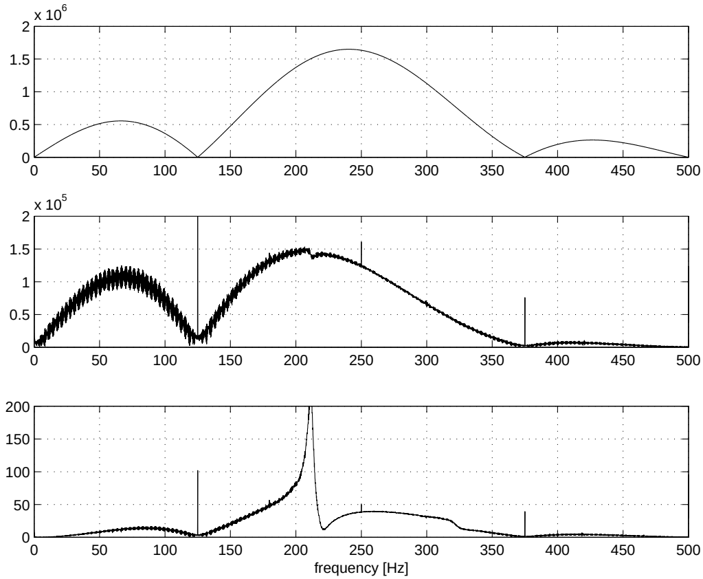
Figure 4: Fourier transforms of drive signals, 2006 Lake Washington test. Top: drive signal from file mp001.sam . Middle: power amplifier drive voltage from file mptest15.sam . Bottom: P.A. drive current from file mptest15.sam . The middle and bottom panels utilize the first m-sequence in the file.
