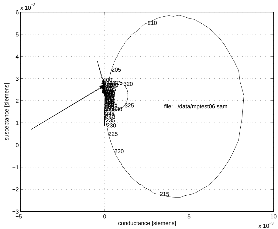
Figure 70: 2006 Lake Washington admittance loop, file MPTTEST06 . DAT
