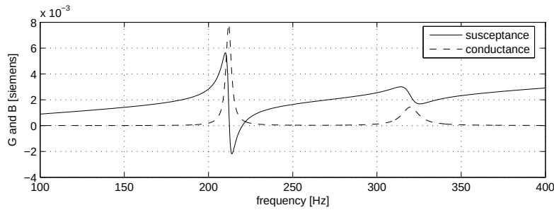
Figure 16: Conductance and susceptance of the circuit, no tuning inductor.
