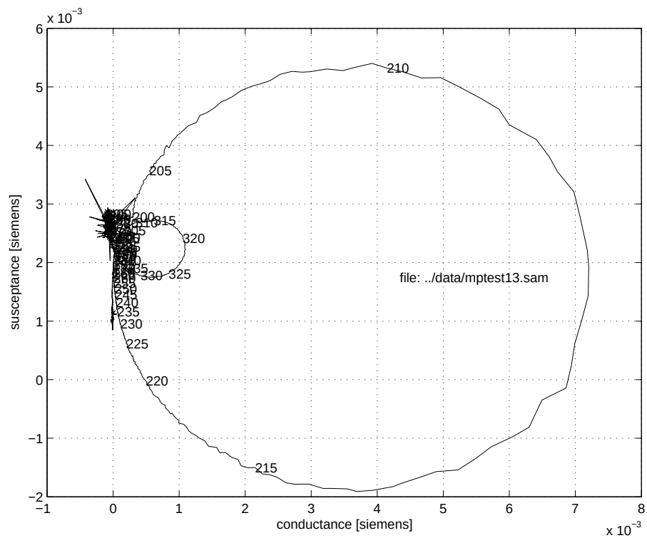
Figure 75: 2006 Lake Washington admittance loop, file MPTTEST13.DAT
