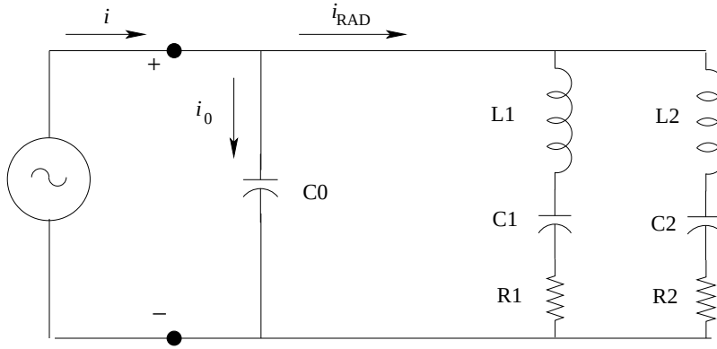
Figure 2: Simple equivalent electrical circuit for the Multiport Source. The “currents” i , i_0 and i_{RAD} are defined in section 2.5.
