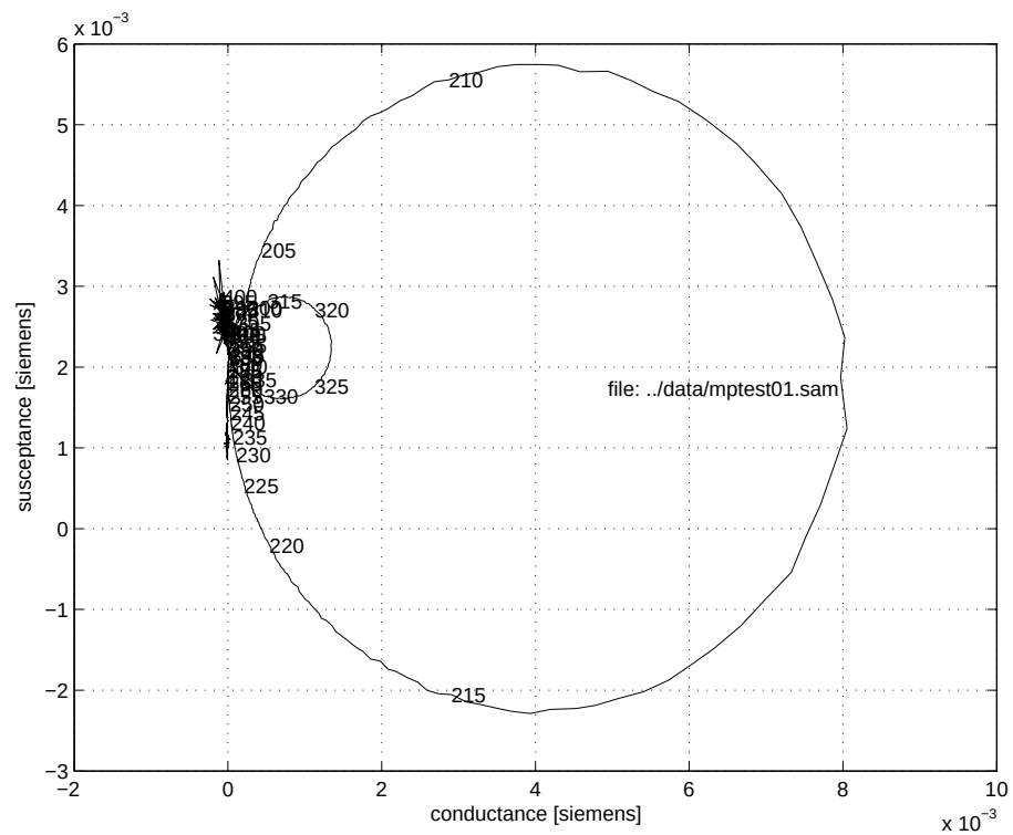
Figure 65: 2006 Lake Washington admittance loop, file MPTTEST01.DAT
