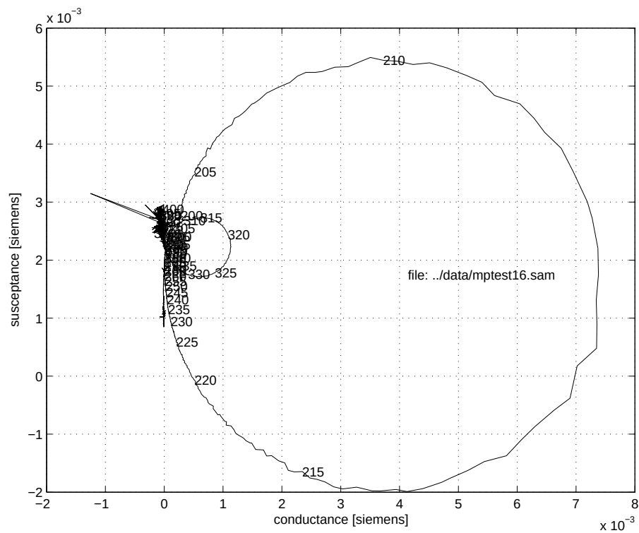
Figure 78: 2006 Lake Washington admittance loop, file MPTTEST16 . DAT
