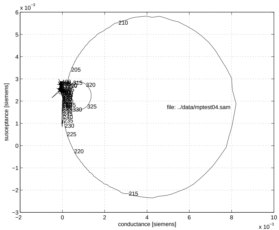
Figure 68: 2006 Lake Washington admittance loop, file MPTTEST04 . DAT
