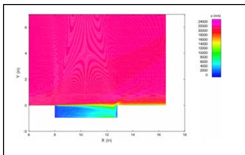
Figure 4 – Time mean of the stream-wise velocities at mid-span
