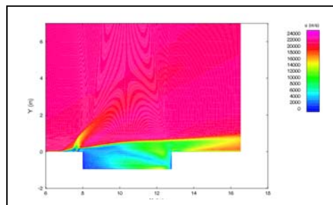
Figure 4 – Time mean of the stream-wise velocities at mid-span
