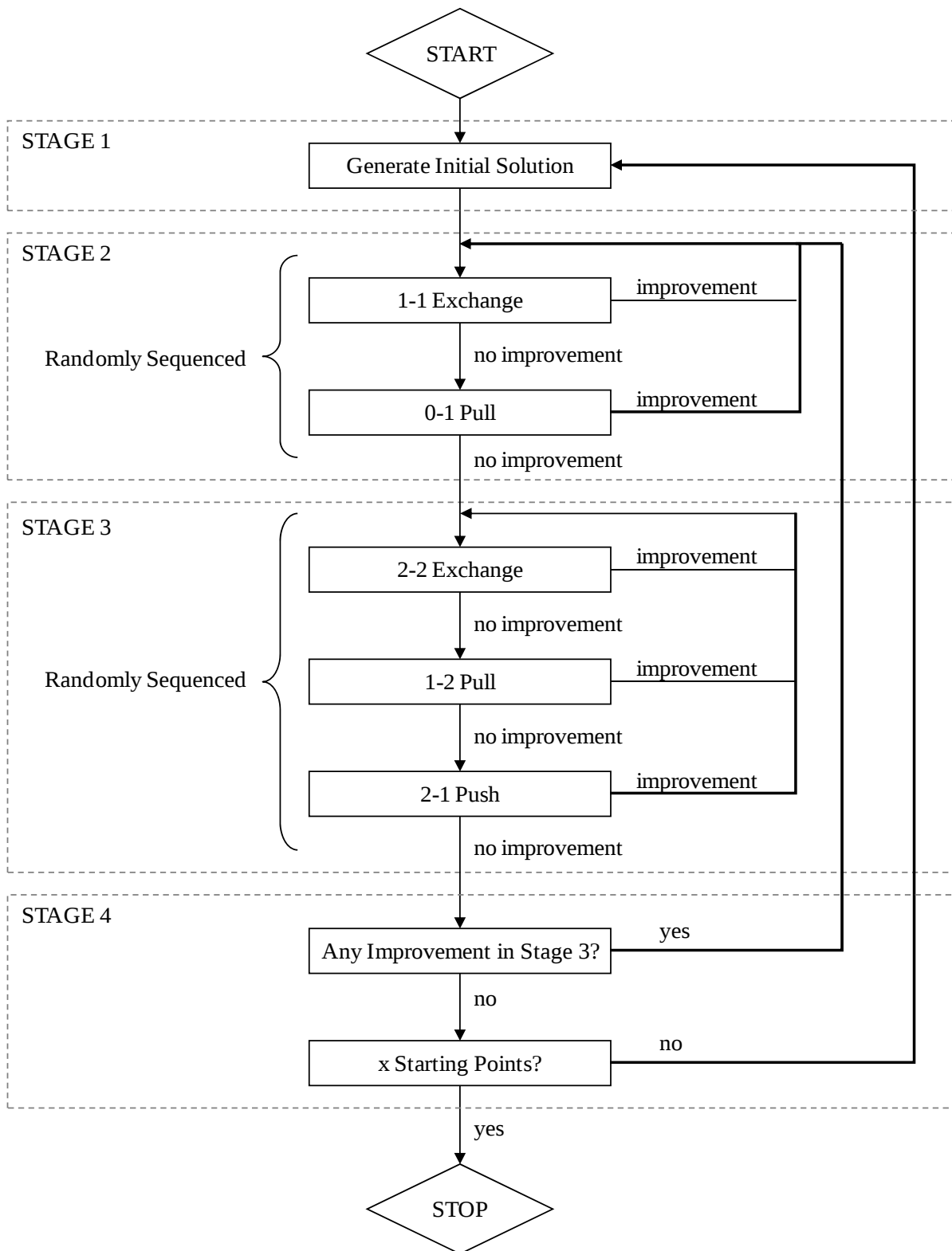
Figure 2. Heuristic Approach
