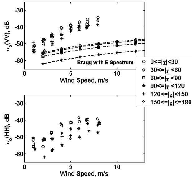
Figure 5. Wind speed dependence of \sigma_0 at various azimuth angles from the wind for the data of 2006. a. \sigma_0(VV) , b. \sigma_0(HH) . Lines show simple Bragg scattering predictions for \sigma_0(VV) using the wind wave spectrum of Elfouhaily et al., 1997; \sigma_0(HH) predicted by Bragg scattering is below the bottom of the lower graph.
