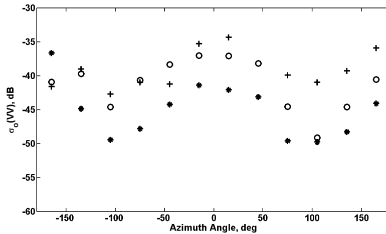
Figure 2. Angular dependence of \sigma_0(VV) at X-band and an incidence angle of 89^\circ \pm 0.25^\circ . These 2005 results are for the ocean surface disturbed only by wind. Symbols are for various wind speeds: + = 4 m/s, o = 6 m/s, * = 8 m/s.
