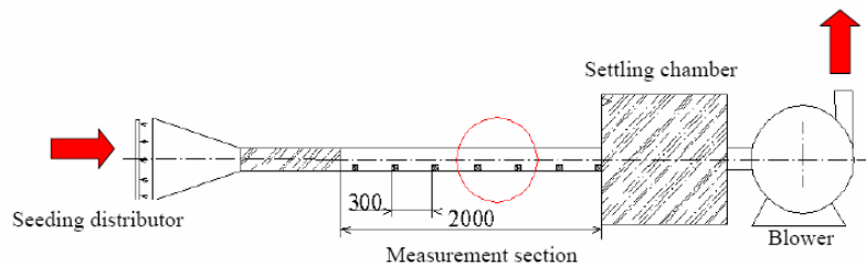
Figure 1: Experimental setup
