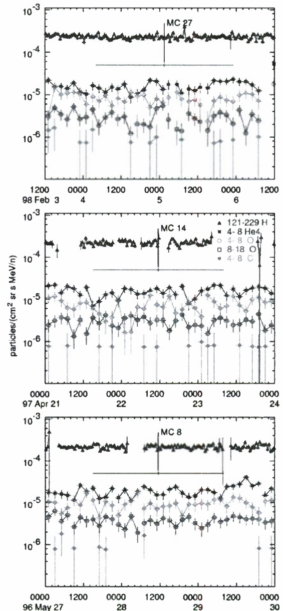
Figure 2. The panels show the intensities of ACR He, C, and O and GCR H in three long duration MC periods.
