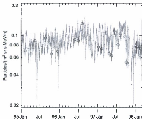
Figure 3. Intensities of 4–8 MeV \text{amu}^{-1} O are shown in MC periods as open circles superposed on the background intensity which is undergoing 27-day variations.
