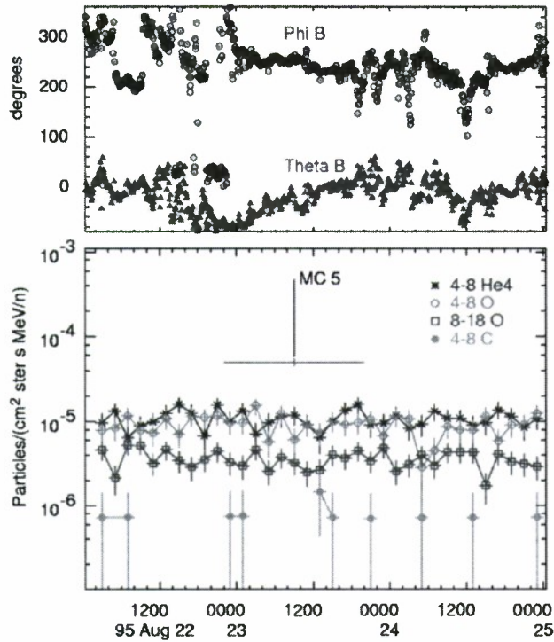
Figure 1. The upper panel shows the polar and azimuthal angles of the magnetic field direction at Wind , in GSE coordinates, showing the uniform rotation during the magnetic cloud indicated as MC 5. The lower panel shows intensities of ACR He, C, and O ions.
