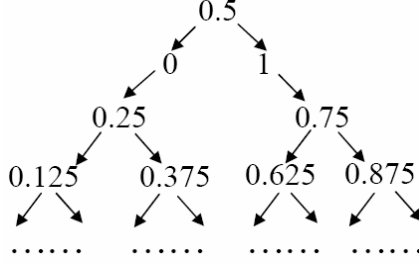
Figure 2: 1D-tree like structure of sparse grid
