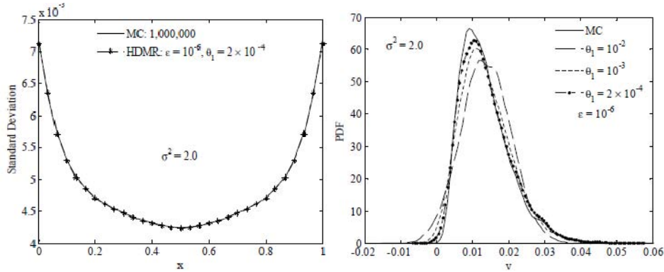
Figure 4: The left figure shows the standard deviation of the v-velocity component across y=0.5 . The right figure shows the convergence of PDF at one point. The problem here refers to flow (squared domain) in random media using and exponential kernel for the log-permeability (with high variability defined by \sigma^2 = 2.0 and 500 stochastic dimensions). The parameter \theta_1 is used to control the adaptive selection of the critical dimensions.
