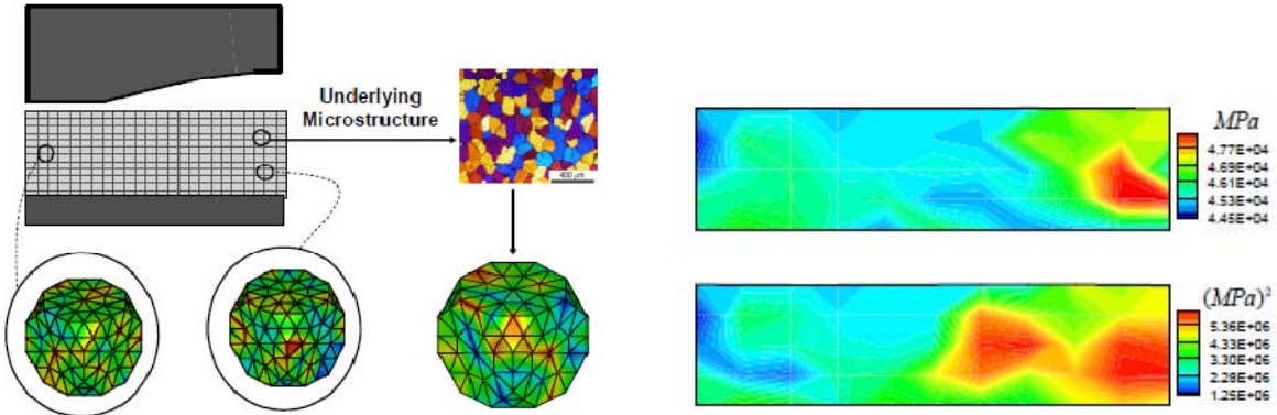
Figure 9: Left: Schematic view of the multiscale problem. Each point on this underlying coarse grid corresponds to a different crystal orientation R . The Rodrigues-Frank axis-angle parameterization is used as a convenient scheme to represent R . Model reduction is conducted simultaneously on the Rodrigues space and the coarse grid. Right: Mean and variance of the shear modulus obtained from the reduced-order representation of texture. This reduced order representation is then used in a stochastic multiscale simulation to compute the variability of properties in the final product (e.g. forged product) induced from the uncertainty in the initial microstructure [9].
