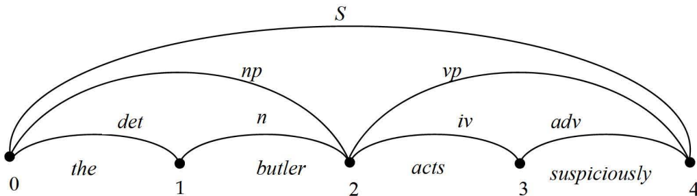
Figure 5: Graph representation
