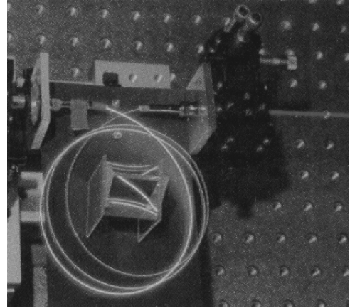
Figure 2. 440 milliwatt fiber laser. Fiber coil diameter is about 5 inches. (Reprinted from Uwe Brinkman, “1.3-kW Fiber Laser Can Be Further Scaled,” Laser Focus World 40, no. 8 [2004]: 2.)
