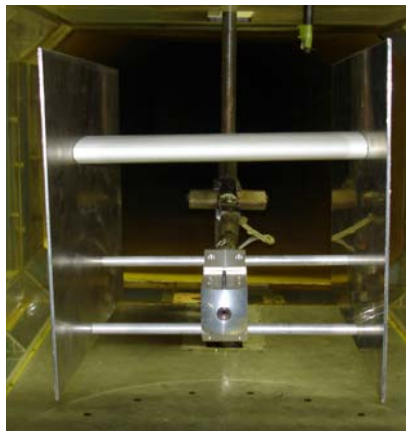
Figure 3. NACA0012 airfoil model mounted on the end plates connected to a sting balance.
