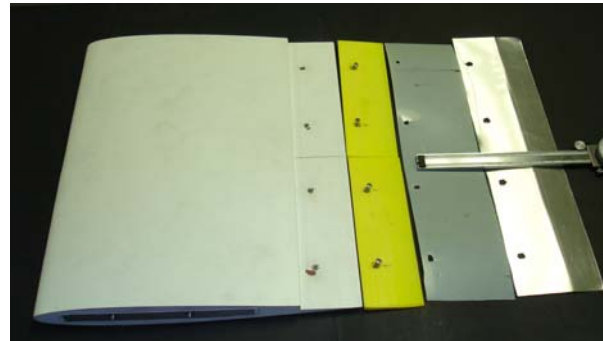
(a) (b) Figure 2. (a) NACA0012 airfoil model with a Mylar SETE, (b) Baseline model, removable parts, and aluminum SETE and Mylar SETE.
