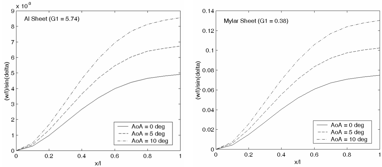
Figure 15. Normalized deformation of the aluminum SETE and Mylar SETE with a deflection angle of 5 degrees for different AoAs.
