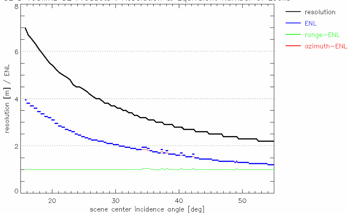
Fig. 12: Spotlight single polarization SE product variant for 100 MHz range bandwidth.
