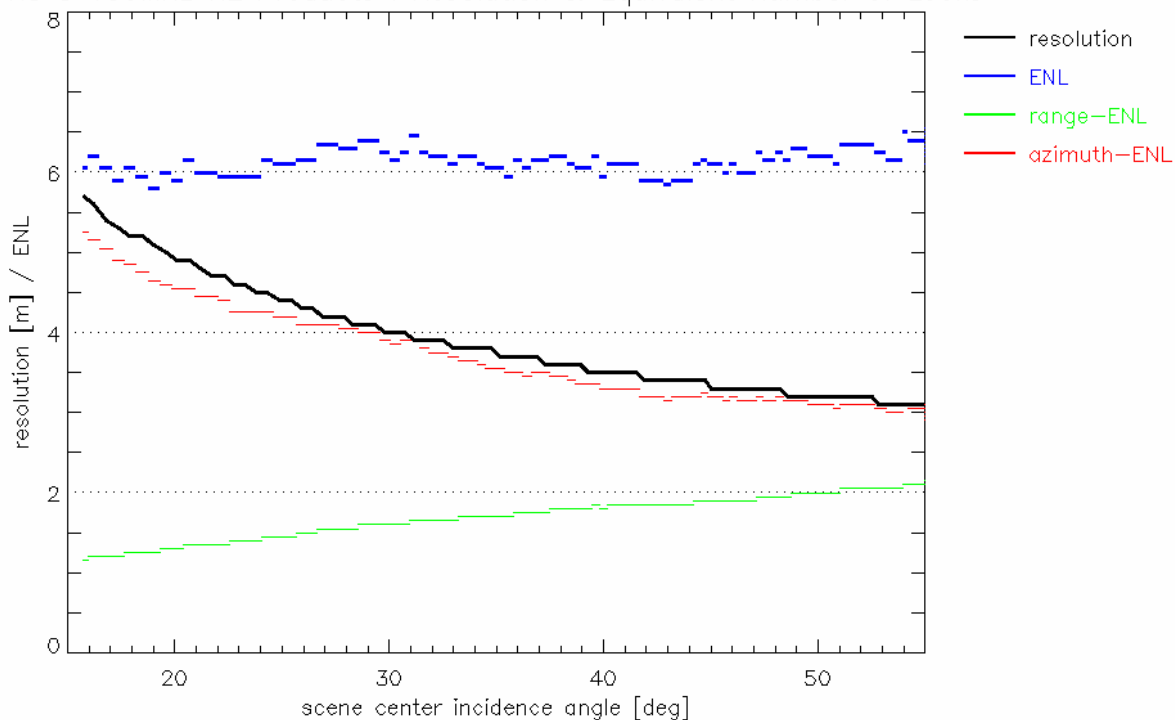
Fig. 19: High-resolution Spotlight single polarization RE product variant for 150 MHz range bandwidth.
