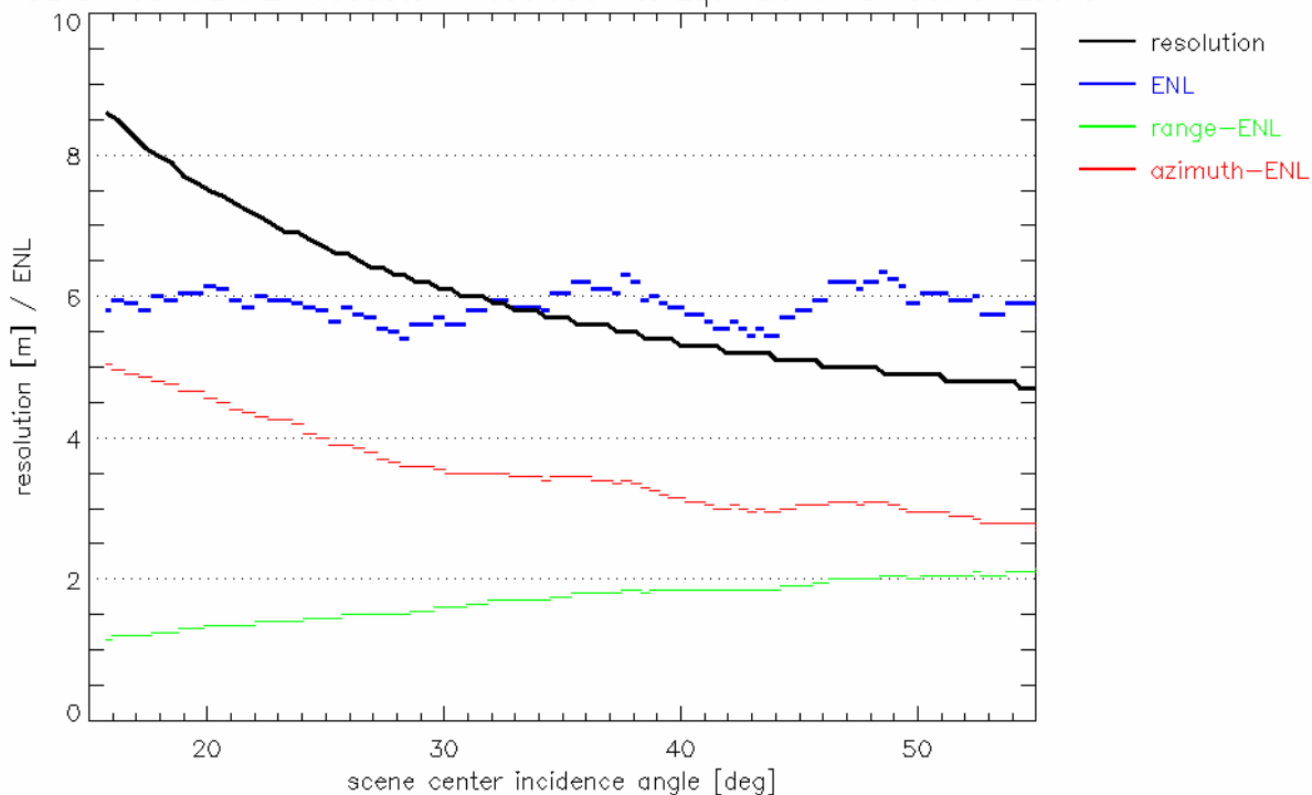
Fig. 11: Spotlight single polarization RE product variant for 100 MHz range bandwidth.
