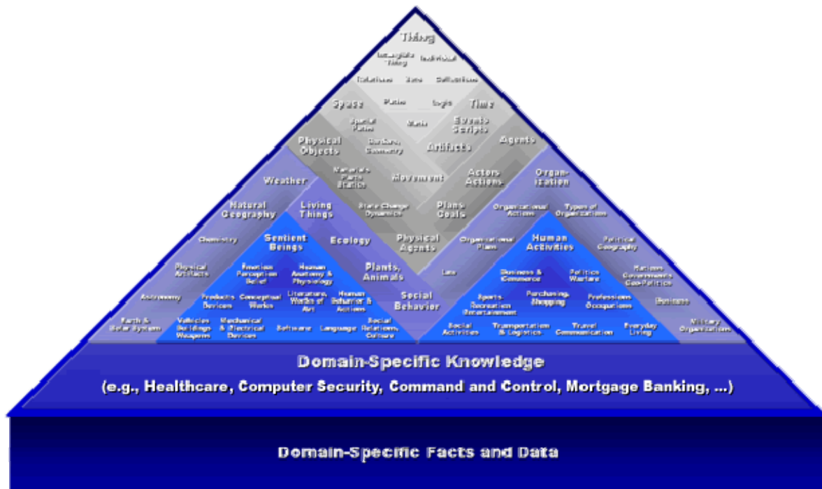
Figure 4: Cyc Ontology
