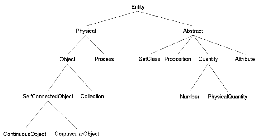
Figure 7: A Subset of Top Level Categories in SUMO [34]
