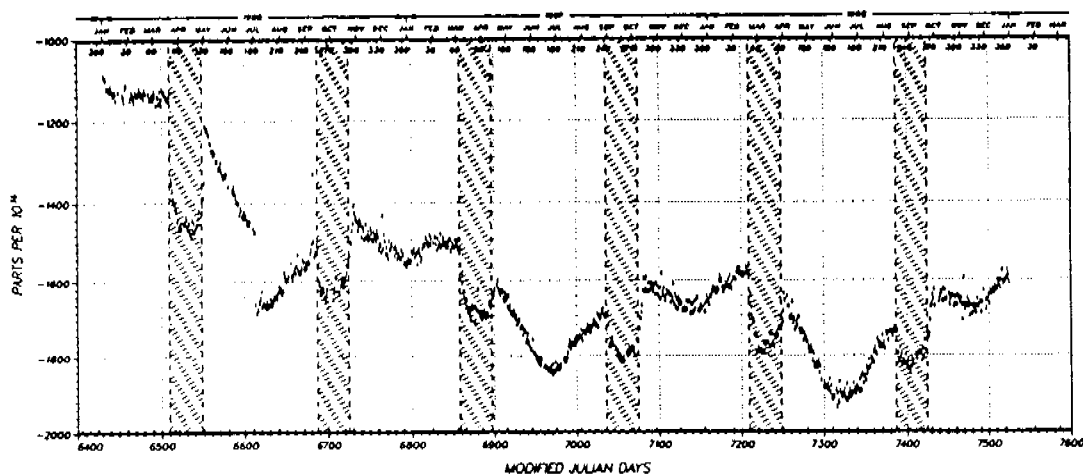
RUBIDIUM OSCILLATOR (NO.19) FREQUENCY OFFSET NAVSTAR 3 versus United States Naval Observatory MC #2 -175 pp10(14) FREQUENCY BREAK @ MJD 6613
