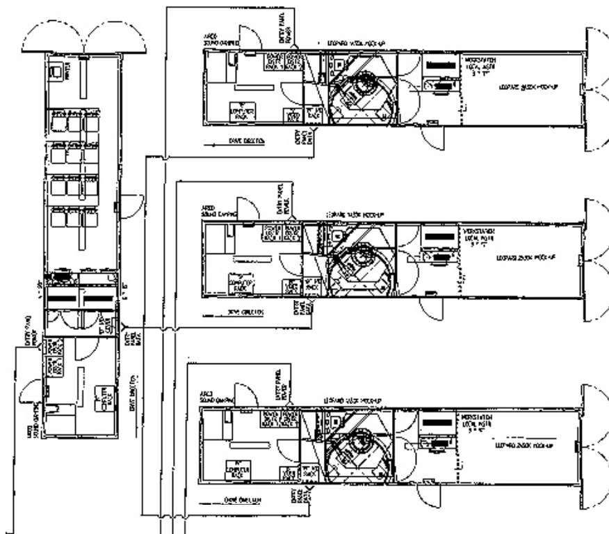
Figure D-37: Tank Simulator.
