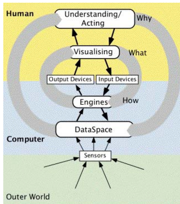
Figure 2-1: The VISTG Reference Model Set in an Environment in which the Computer Acquires Data Autonomously from an Outer World of Interest to the Human User. The conceptual information flows follow the thick grey arrow loops, but the physical information flows must follow the paths marked with small black arrows. When applied to a real system, each arrow may represent multiple parallel paths and possibly many levels of structure.
