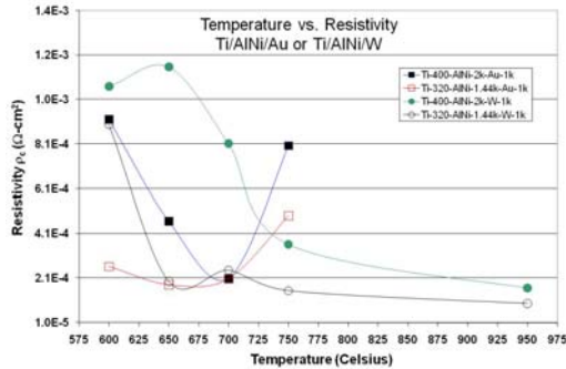
Fig.1 The effect of anneal temperatures on specific contact resistivity
