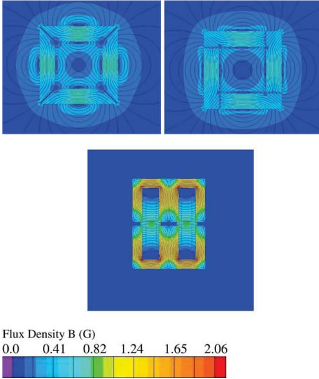
Fig. 4. Flux density map for normalized inductor models (CW from top left: square 45° gap core, square 90° gap core, E-E core, and legend).
