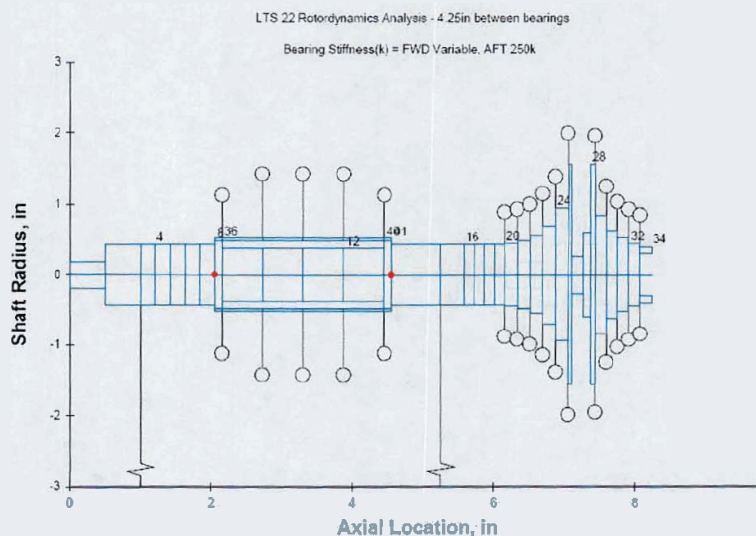
Figure 19 LTS22 Rotor System Model
