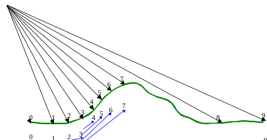
Figure 5. A single vertical scan-line detecting the ground. Pixel 0 is altered to correspond to the bottom of the vehicle wheel. Pixels 1, 2, 3, 8 and 9 are ground pixels due to shallow slopes. Pixel 4, 5, 6 and 7 are obstacles due to steeper slopes. The slopes are shown by the direction vectors on the bottom of the figure.
