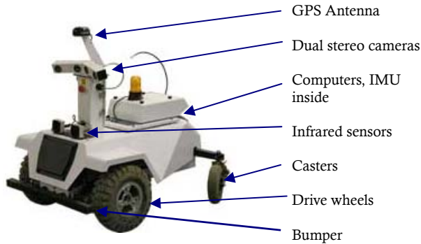
Figure 2. The DARPA LAGR vehicle
