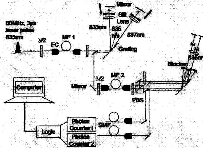
Fig. 2. Schematic experimental setup. PBS: polarizing beam splitter, SMF: single mode fiber, \lambda/2 : half-wave plate. MF1 and MF2 are microstructure fibers.
