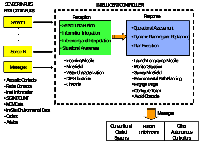
Figure 1: High Level Decomposition for a Single IC.
