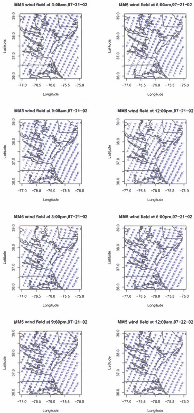
Figure 4: Wind field maps, showing wind direction and speed.
