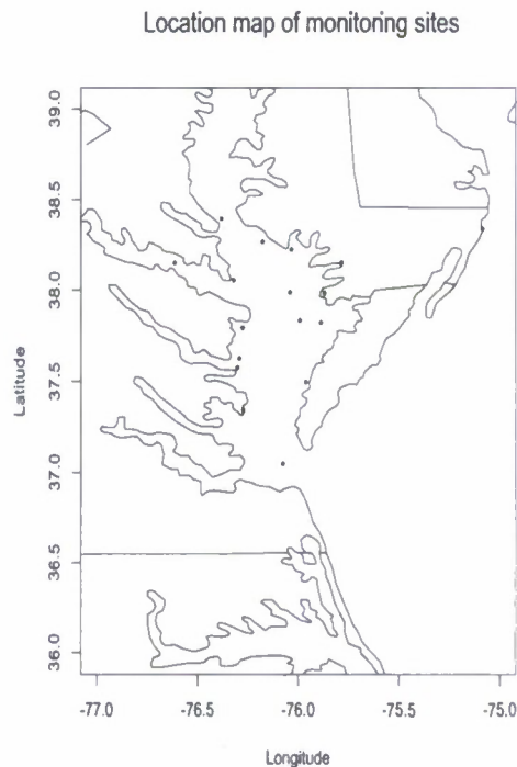
Figure 2: The location map of monitoring sites.
