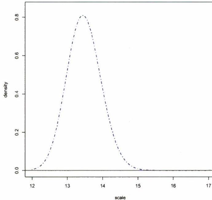
Figure 10: Posterior distribution for the scale parameter.
