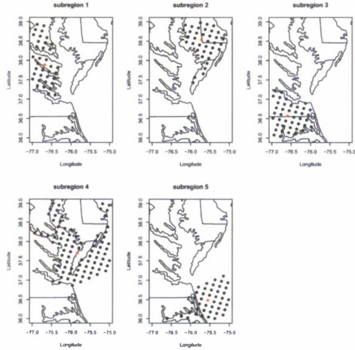
Figure 5: Subregions of stationarity.
