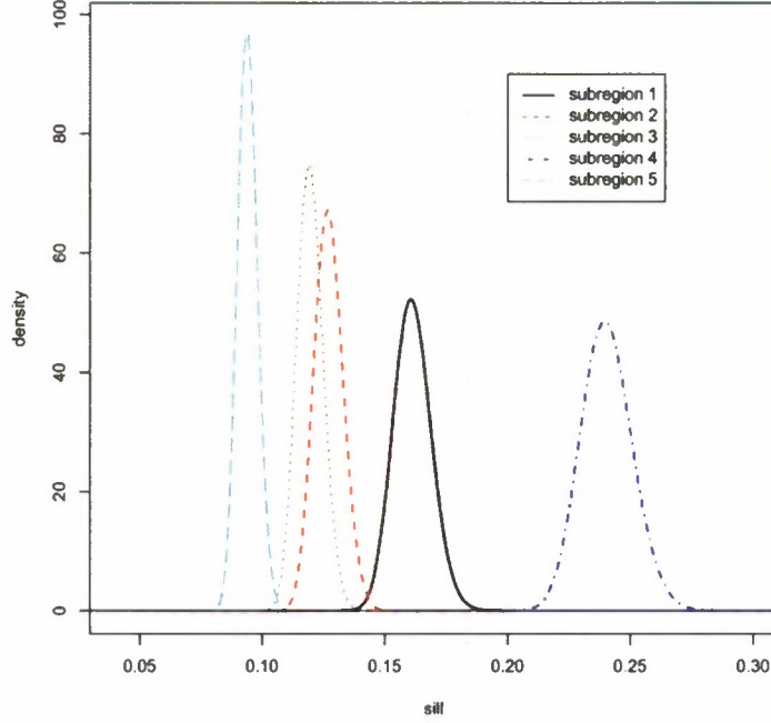
Figure 8: Posterior distribution for the sill parameter.
