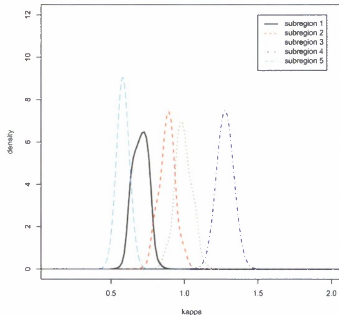
Figure 11: Posterior for smoothness parameter.
