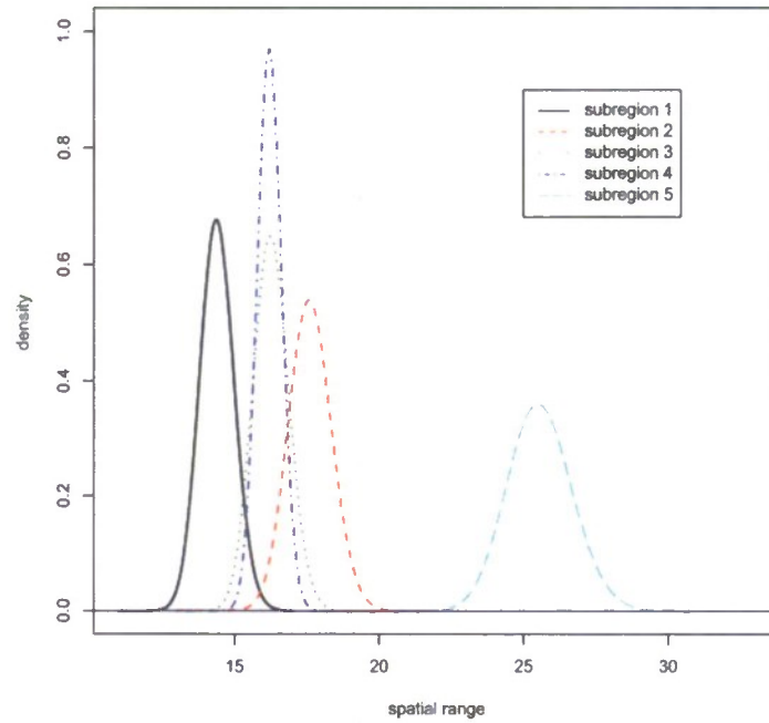
Figure 9: Posterior distribution for the spatial range.
