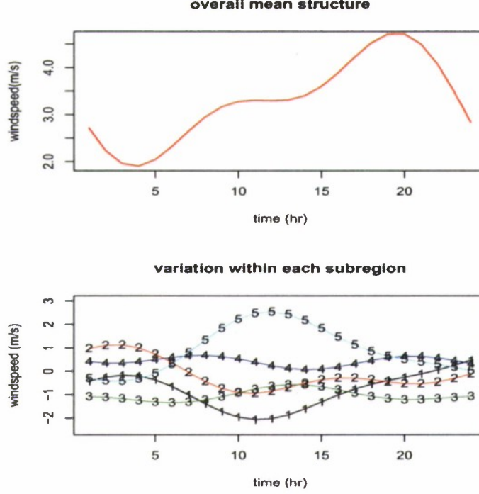
Figure 6: Spatial-temporal trend for wind speed. Top graph (a): overall temporal trend. Bottom graph (b): mean temporal variation for each subregion.
