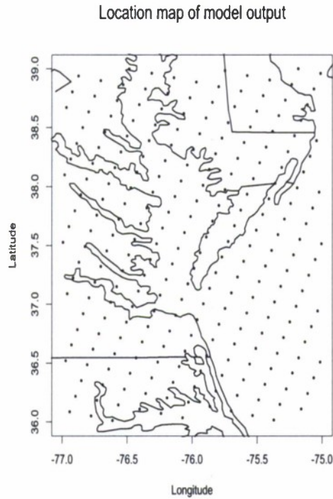
Figure 3: Grid for MM5 output.
