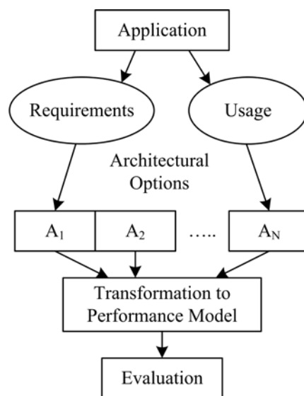
Figure 3: Framework Architecture
