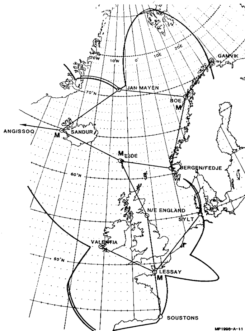
Figure 2: Loran-C European possible coverage about 1995
