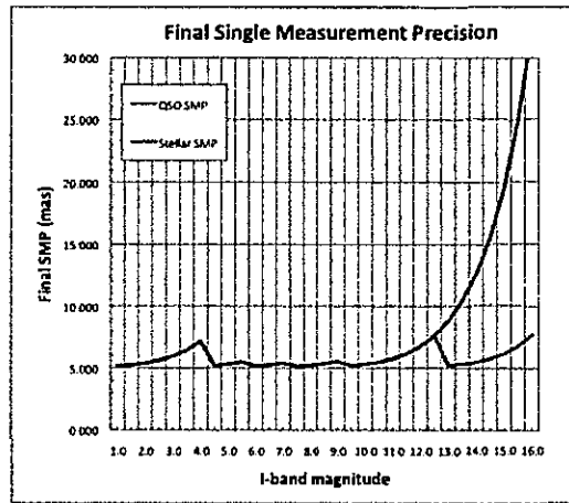
Figure 5: JMAPS single measurement precision predictions as a function of stellar I-band magnitude
