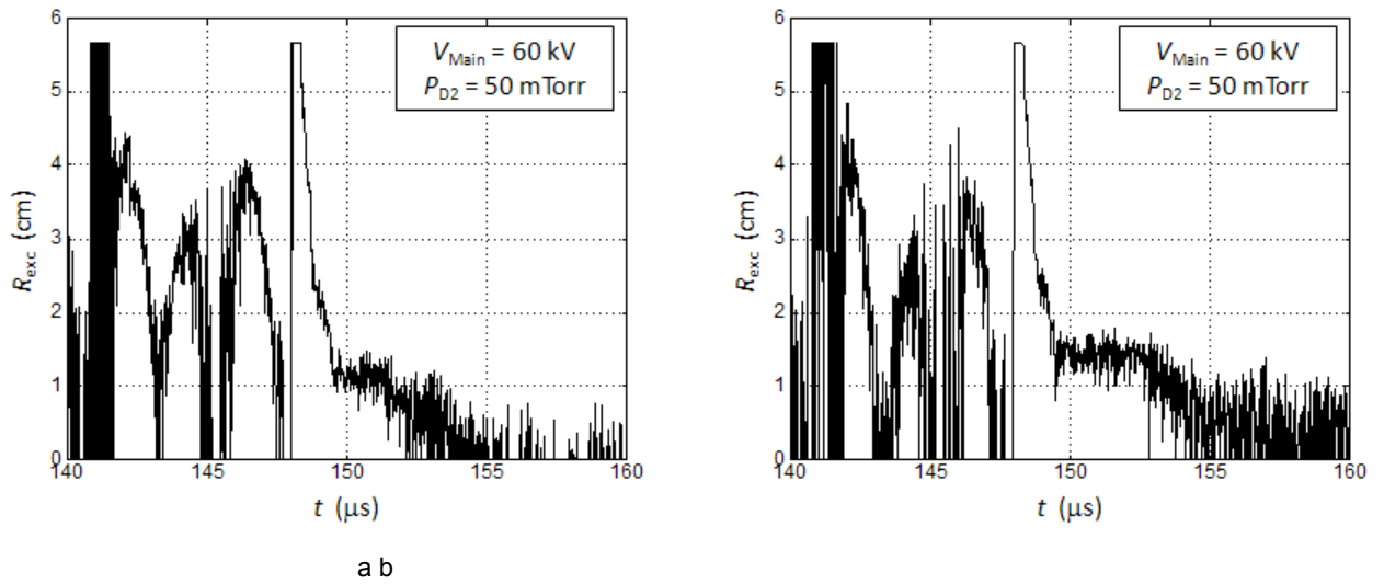
Figure 92. Excluded flux radius vs. time calculated at (a) Theta coil segment D; (b) Theta coil segment G
