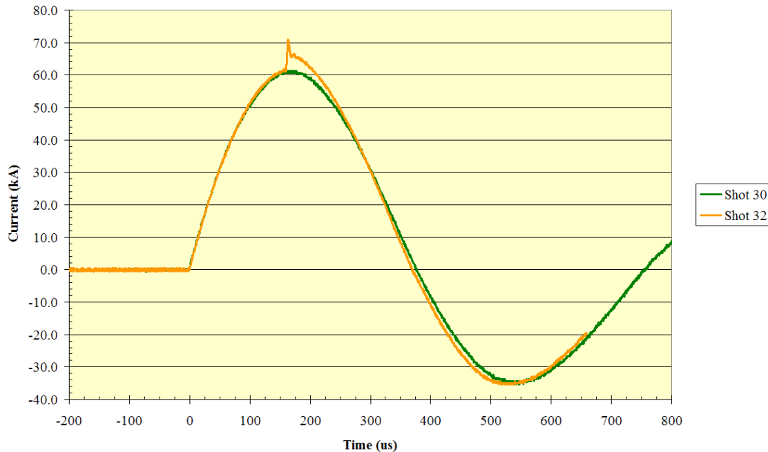
Figure 5. Bias bank current waveforms recorded with Bias Pearson monitor
