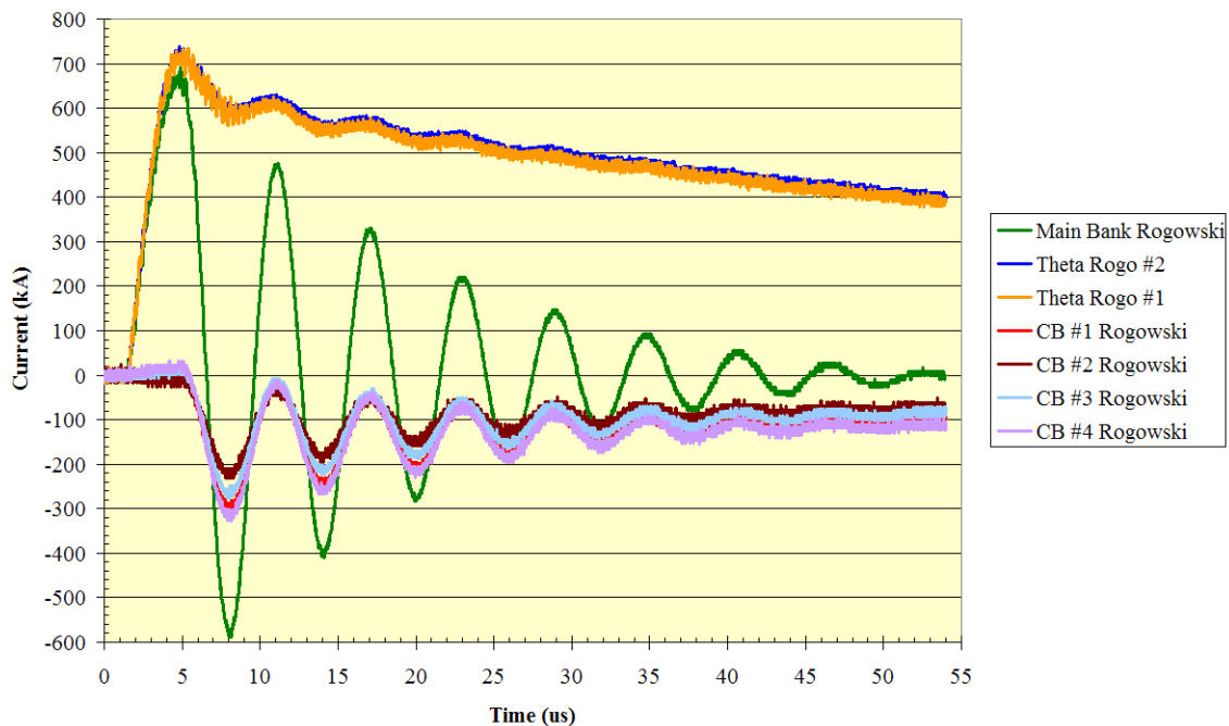
Figure B11. Current waveforms obtained from Main bank, Theta coil, and Crowbar rail-gap Rogowski coils
