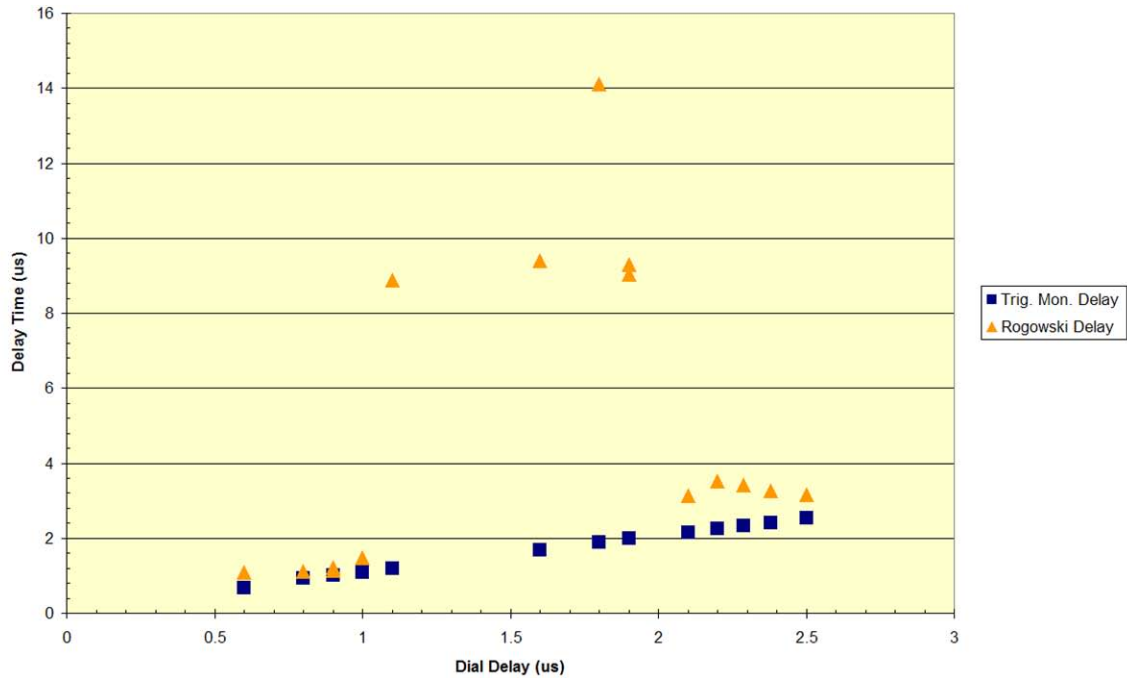
Figure B4. Trigger monitor and Rogowski coil delay data from Table B2 vs. intended delay set by the delay generator ("Dial Delay")
