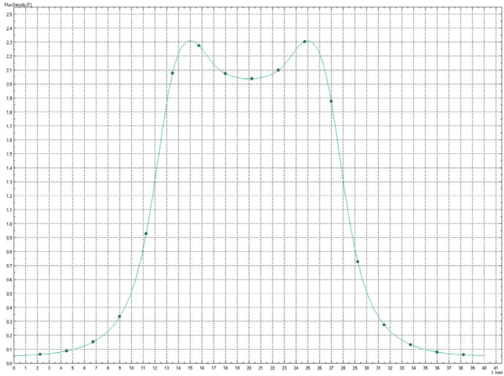
Figure A4. Magnetic flux density at r = 0 cm (on axis) vs. axial position
