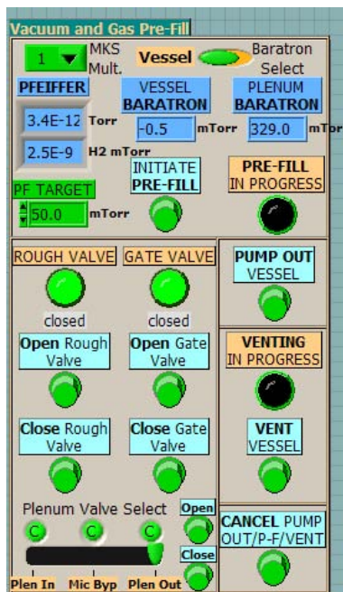
Figure 79. Vacuum-system controls on control program's front panel
