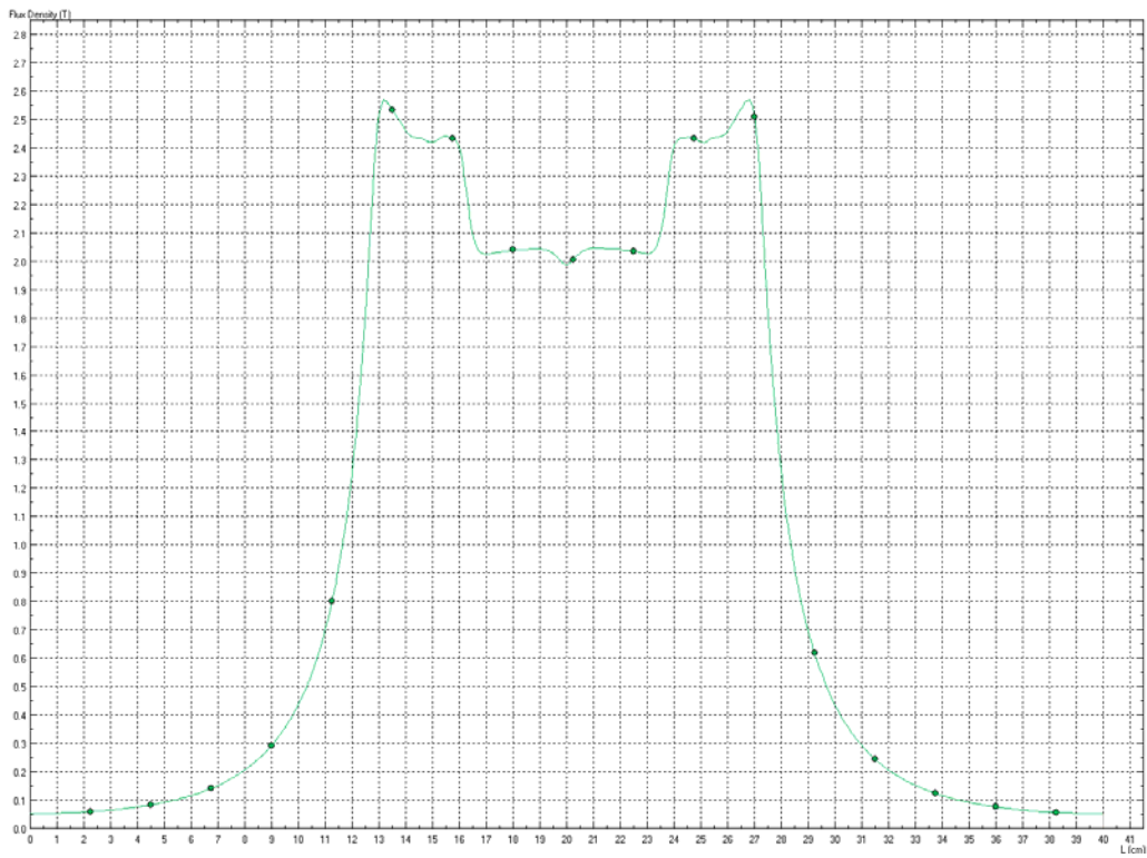
Figure A5. Magnetic flux density at r = 2.0 cm vs. axial position
