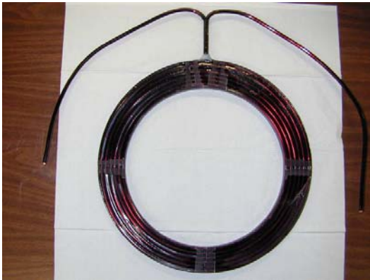
Figure 101. (a) First mirror coil; (b) several coils in G-10 spools
