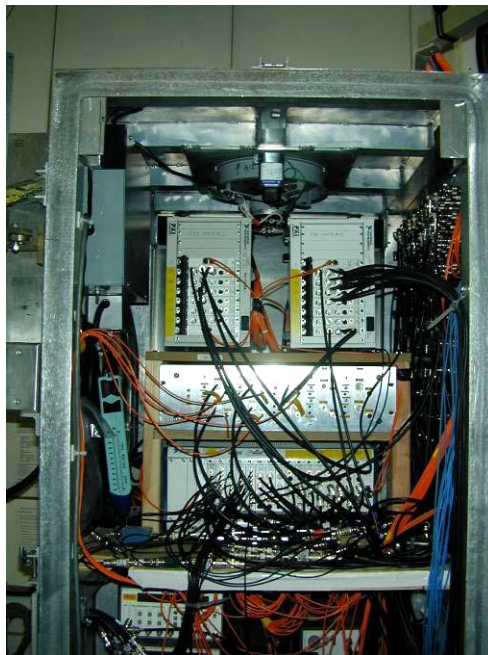
Figure 58. Trigger sync-out receiver box positioned among PXI digitizer crates
