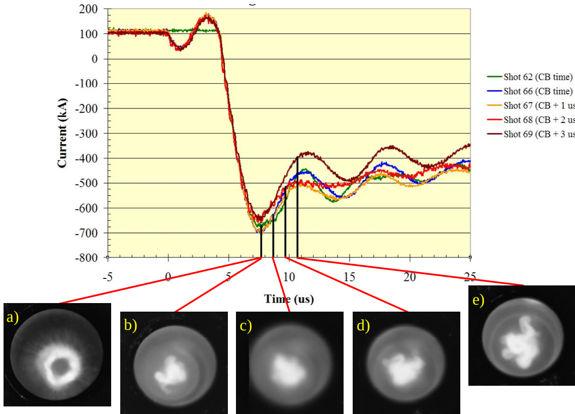
Figure 32. Theta coil current, along with five MCP camera images
