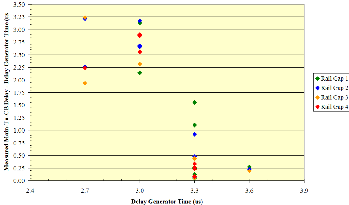
Figure B13. Delay between Crowbar rail-gap trigger and start of conduction vs. desired Main-to-Crowbar delay
