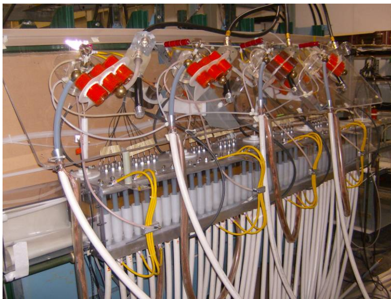
Figure 25. Auxiliary bank to be used to augment trigger pulse delivered to each Crowbar rail gap. It was decided later to abandon these tests in favor of doubling up the charged trigger cables on all four of the Crowbar rail gaps, a scheme that was tested during the Phase II effort for FRCHX and that, in fact, was finally successful in ensuring that all four Crowbar rail gaps conducted reliably during each shot. For further discussion of this scheme, see Section 4.6.2.
