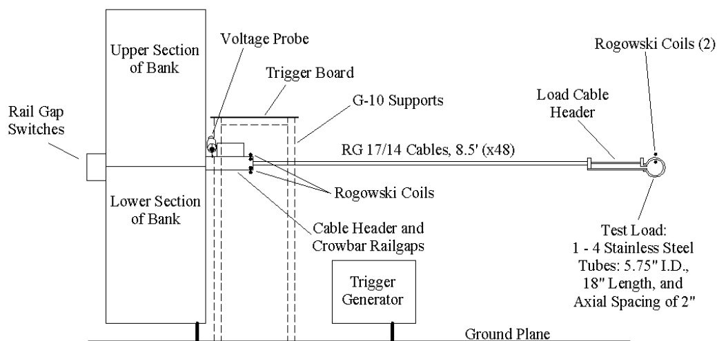
Figure B1. Test setup for crowbar switch
