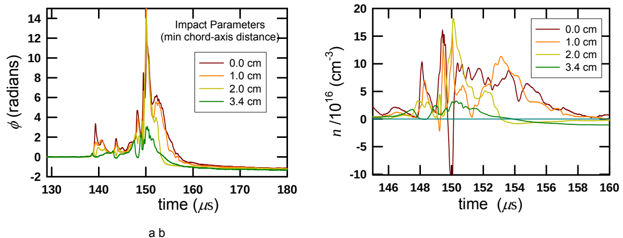
Figure 90. Interferometer data: (a) phase shift as a function of time; (b) corresponding line-integrated density
