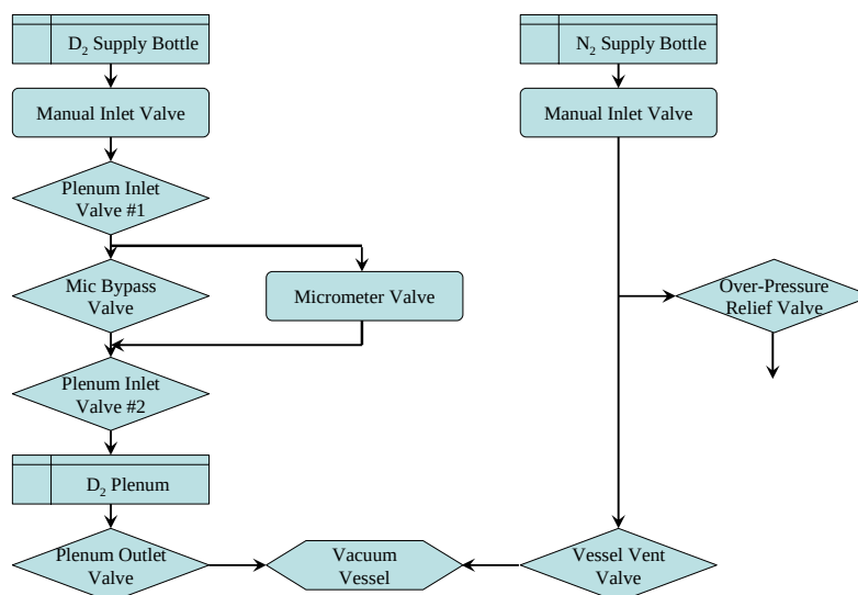
Figure 50. D 2 pre-fill and N 2 venting systems for FRCHX vacuum vessel
