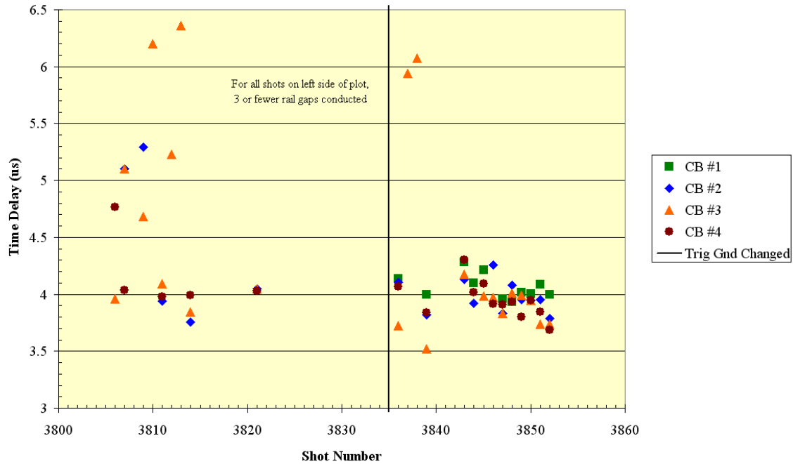
Figure B8. Delay between start of Main bank current and start of current in Crowbar rail gaps. Somewhat erratic current start times were observed right before the change in the crowbar trigger circuit grounding. Such erratic behavior does not appear to have been always the case, though. Figure B9 adds a few data points from a shot taken quite some time ago.
