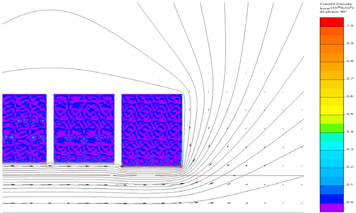
Figure A2. Calculated current density in field-coil segments
