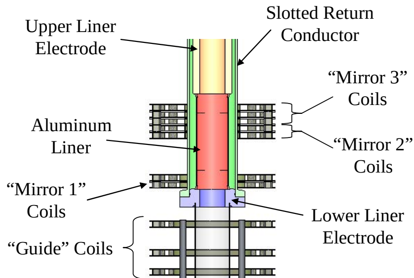
Figure 100. Guide and Mirror coil assembly around solid liner
