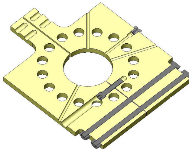
Figure 105. Theta coil segment, showing location for adding a third bolt
