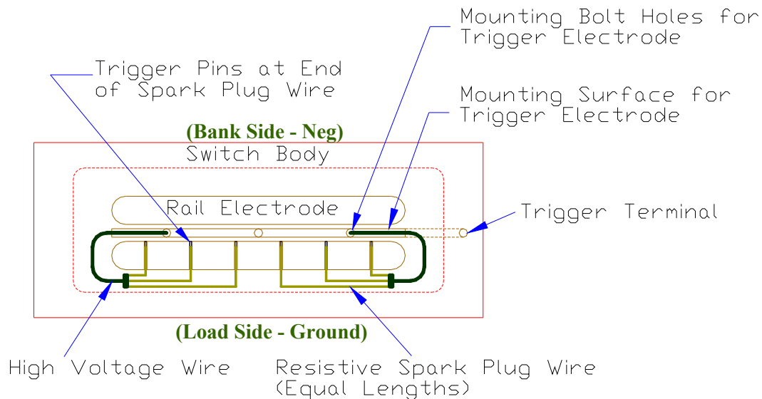
Figure C5. Vacuum rail-gap switch concept
