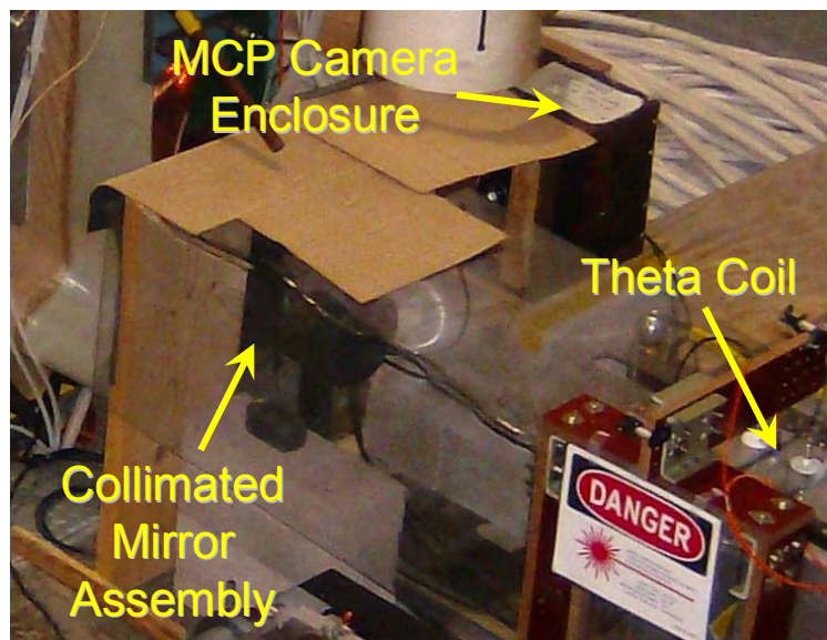
Figure 14. MCP camera setup at north end of quartz tube
