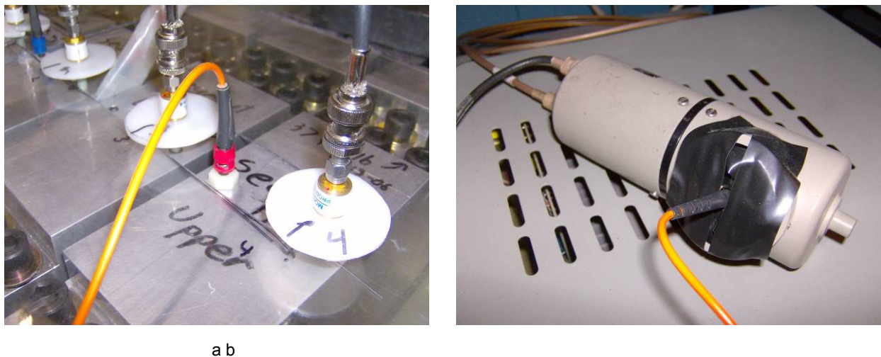
Figure 13. First light fiber monitor (a) mount on Theta coil; (b) PMT detector in screen room
