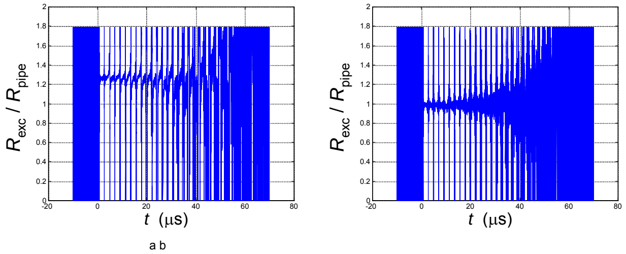
Figure 81. Excluded flux radius to pipe radius for 12-cable setup using (a) short time-scale integrators; (b) long time-scale integrators
