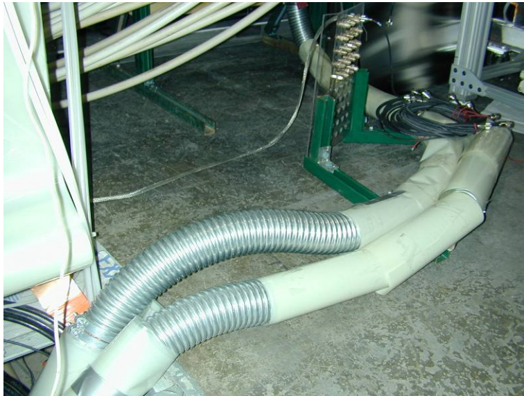
Figure 61. Conduit attached to ends of rigid conduit exiting cable trays
