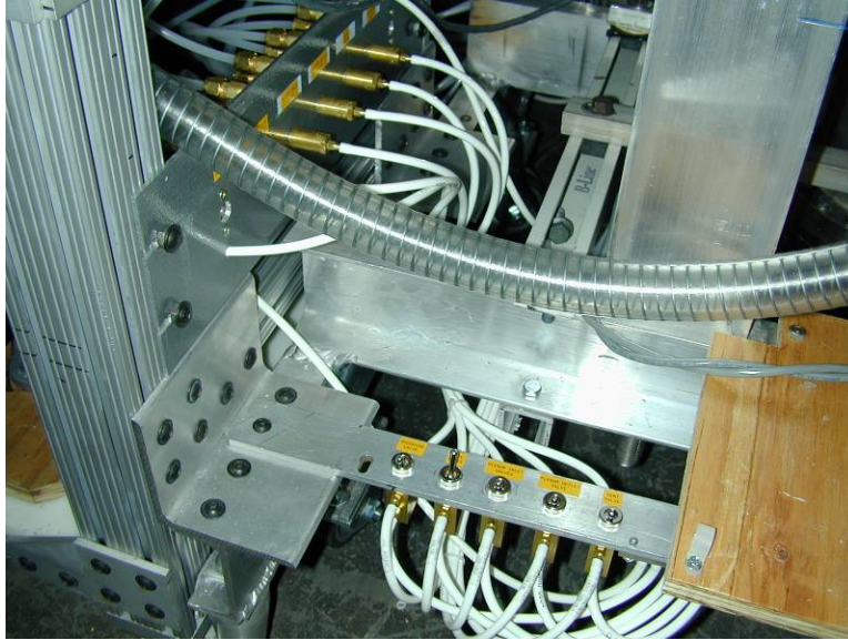
Figure 74. Pneumatic control valves and their manual toggle switches
