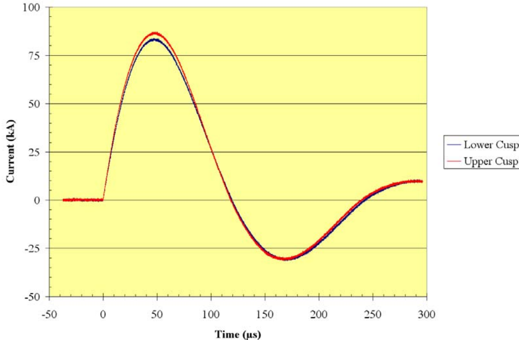
Figure 85. Upper and Lower Cusp current waveforms from test #7, 5 Mar 2008.
