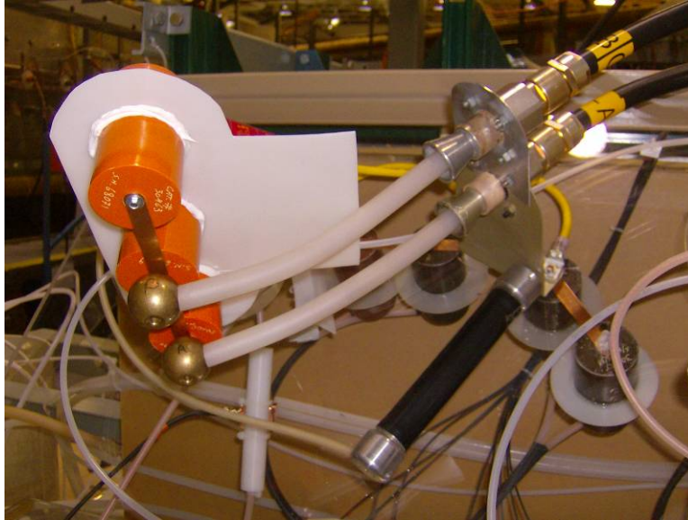
Figure 24. Trigger-board-circuit setup for end-rail-gap-only tests
