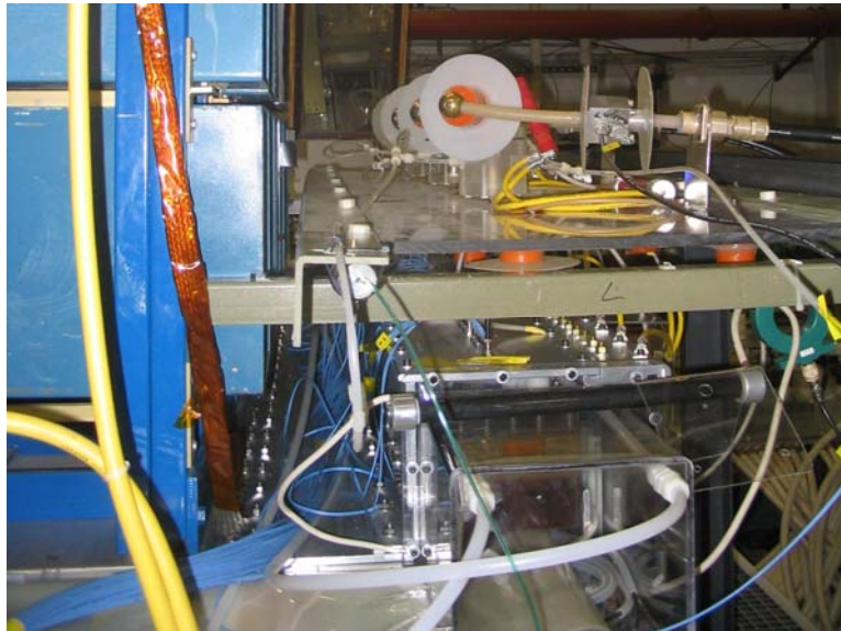
Figure C4. FRX-L Crowbar switch showing its close proximity to Main bank
