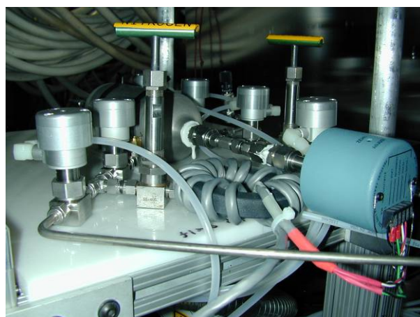
Figure 51. (a) D 2 pre-fill; (b) N 2 backfilling and venting system components
