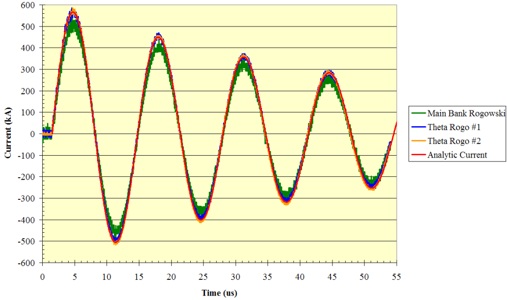
Figure 9. Current waveforms obtained from Rogowski coils on Main bank and on current feed to Theta coil
