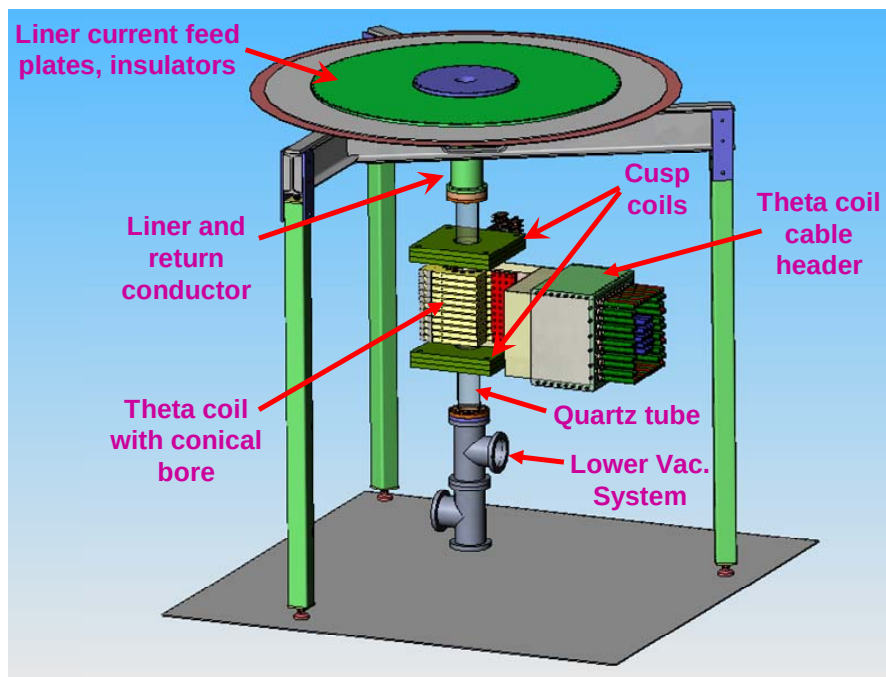
Figure 109. Layout for FRCHX formation and translation sections with solid liner
