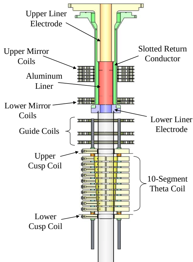
Figure 110. FRCHX formation, translation, and liner-compression regions
