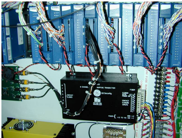
Figure 73. IFS 8-channel contact transmitter in Hammond enclosure
