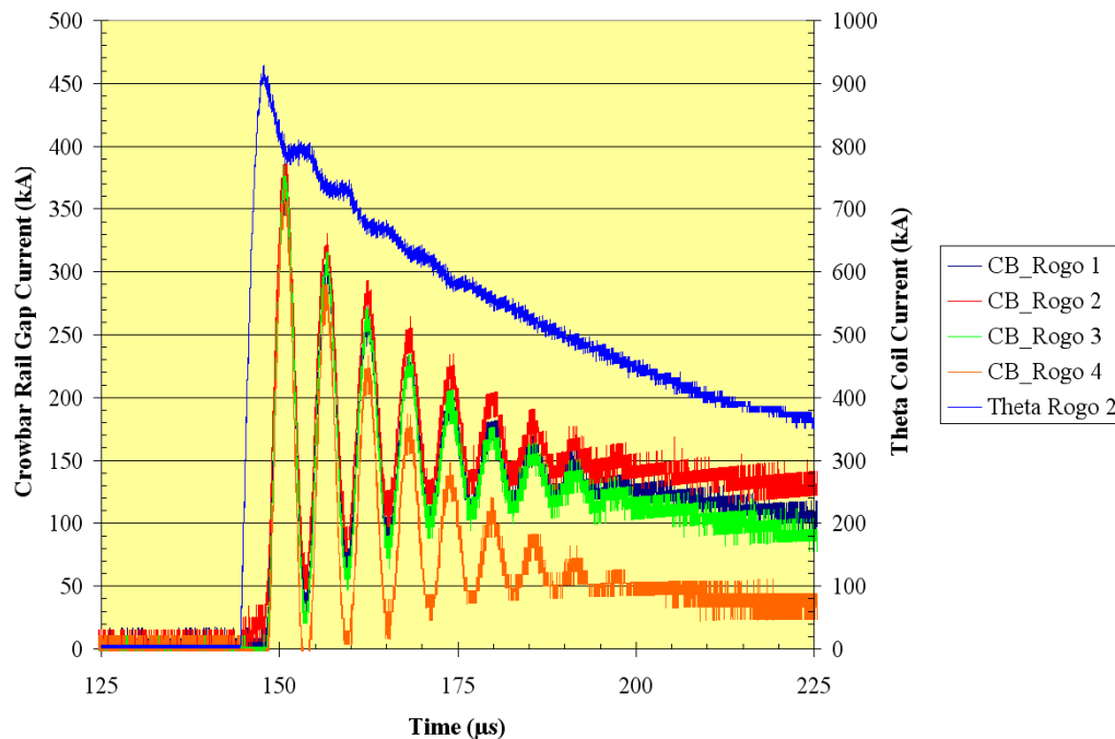
Figure 84. Theta coil and Crowbar rail gap current waveforms from test #9, 3 Mar 2008
