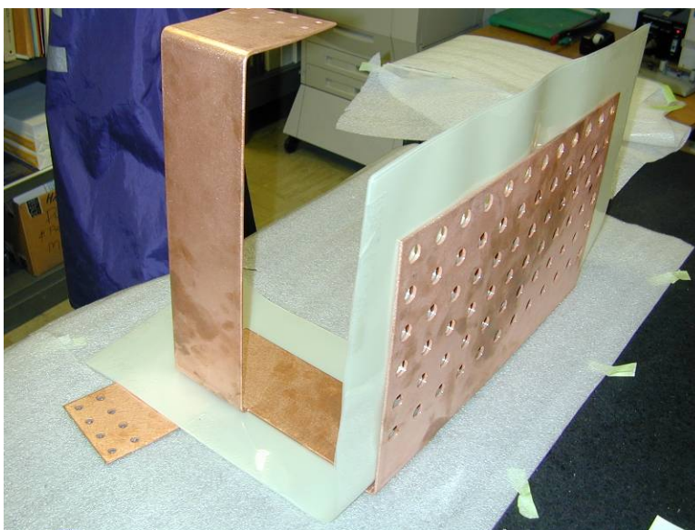
Figure 103. Guide/Mirror coil cable header along with Mylar pack prepared for it
