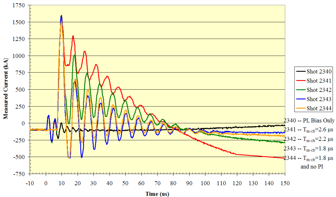
Figure B5. Overlay of several FRX-L Theta coil current waveforms from several shots with varying Main bank-to-crowbar triggering delays
