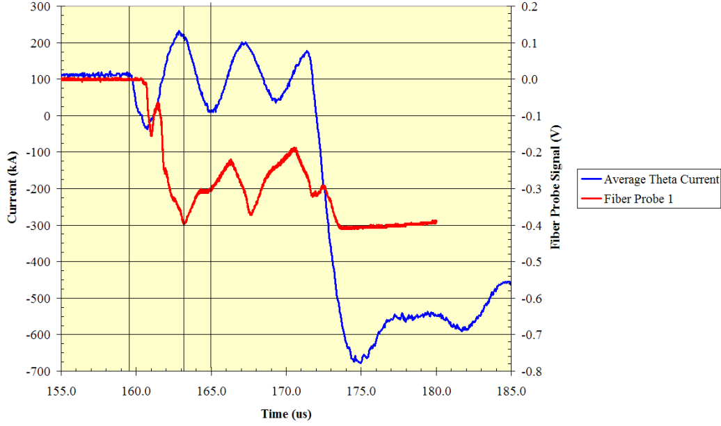
Figure 33. First light fiber-monitor signal with Theta coil current overlaid
