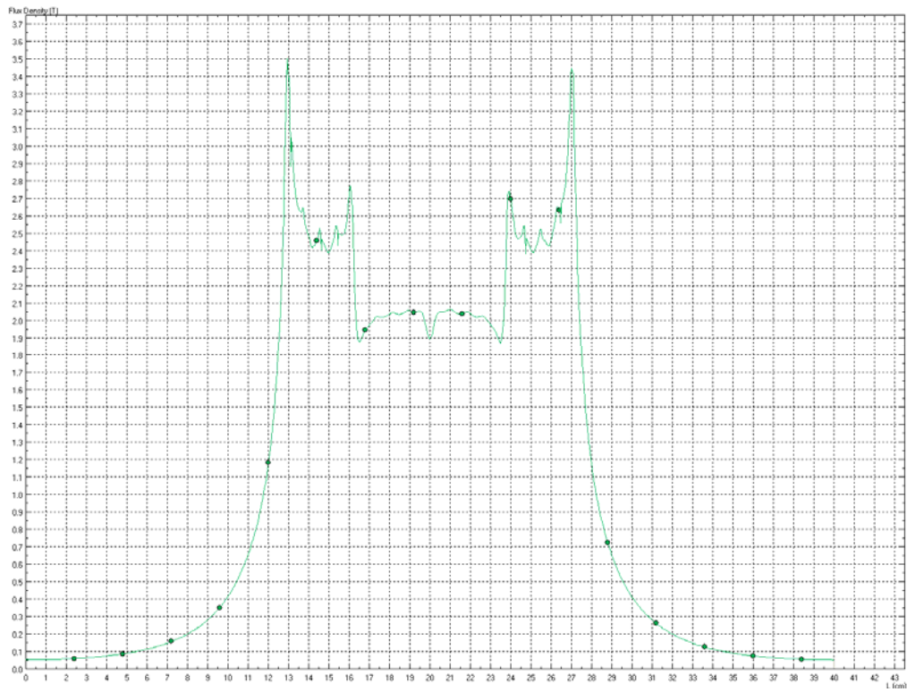
Figure A6. Magnetic flux density at r = 2.3 cm vs. axial position
