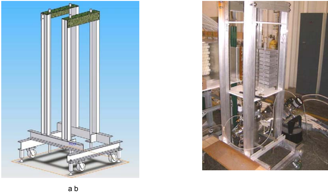
Figure 42. (a) FRCHX vertical support stand; (b) stand after assembly
