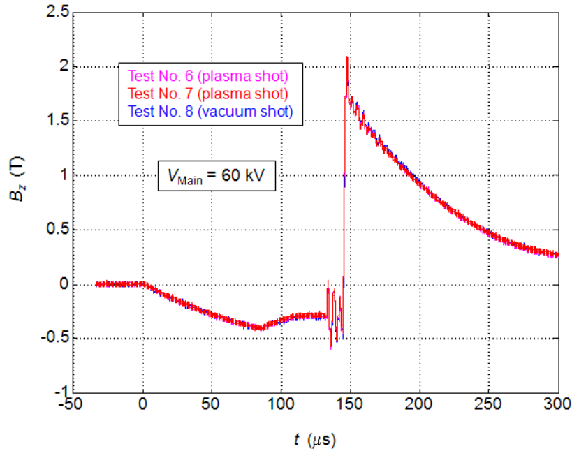
Figure 86. G-segment B-dot probe waveforms from three successive shots, 7 March 2008
