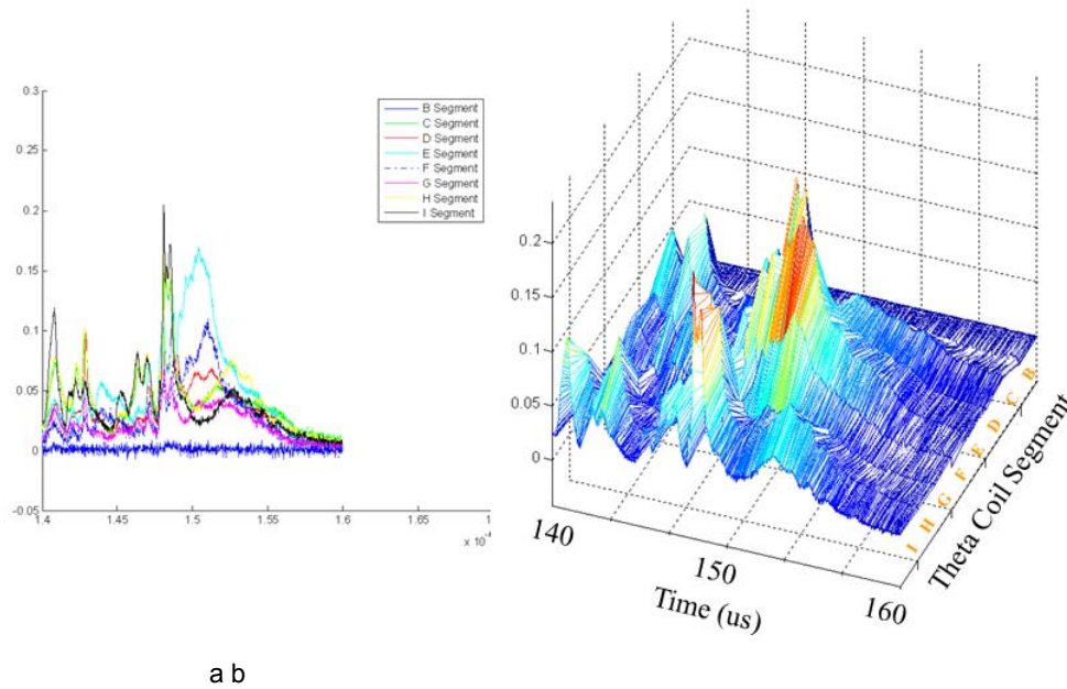
Figure 93. Side-on fiber-optic-array data: (a) signal intensity vs. time; (b) surface plot
