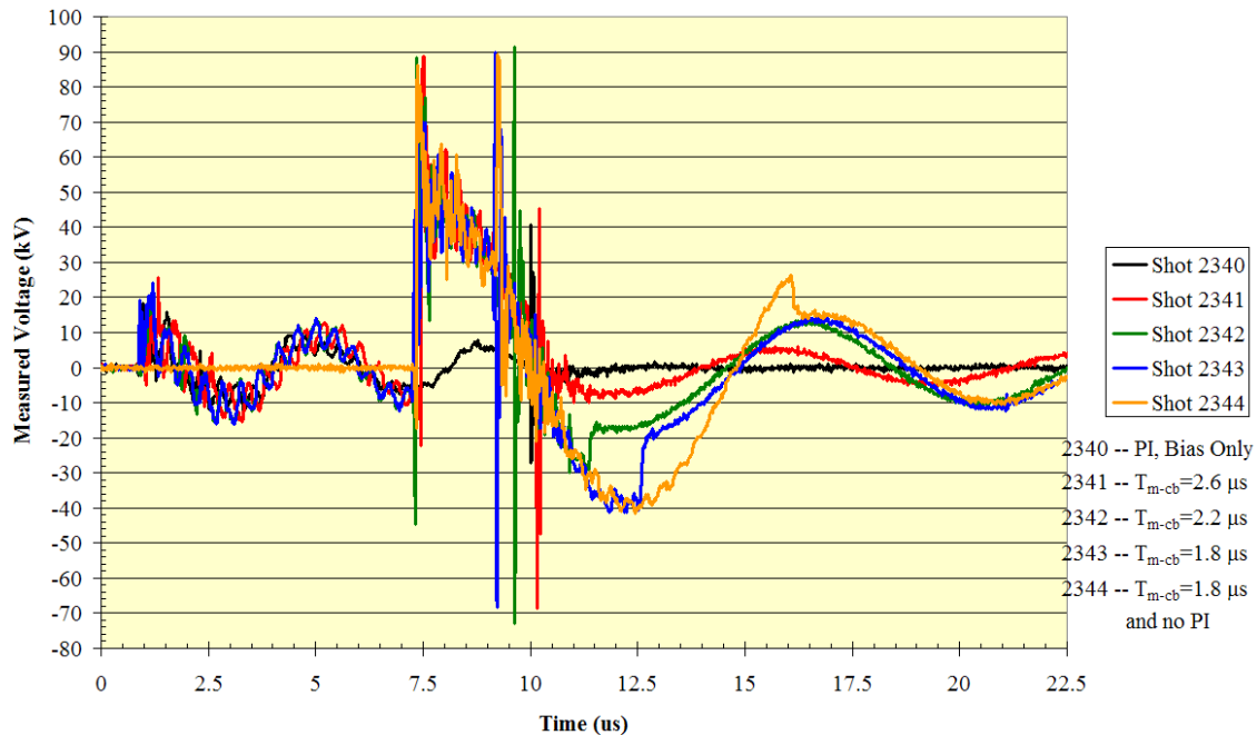
Figure B7. Voltage across the Crowbar switch vs. time
