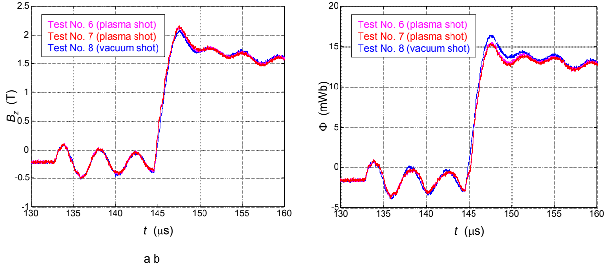
Figure 88. G-segment (a) B-dot probe and (b) flux loop waveforms
