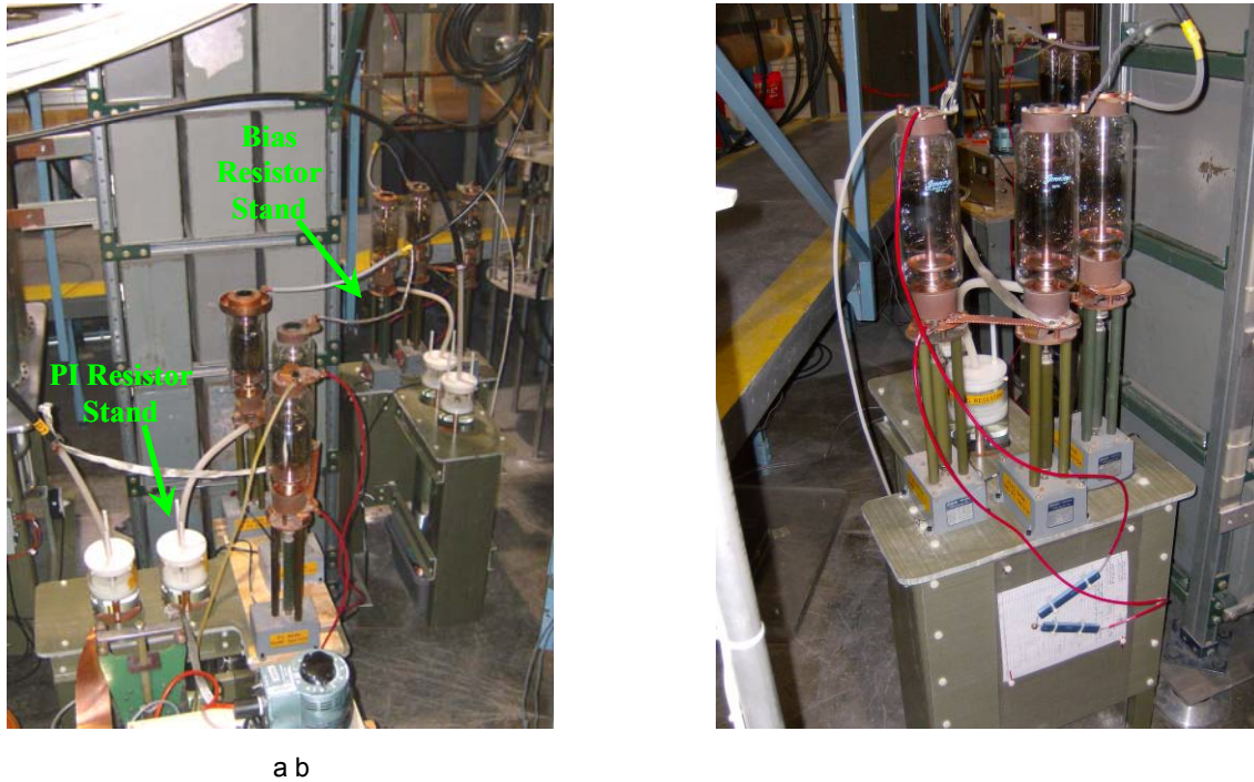
Figure 4. (a) PI and Bias bank resistor stands; (b) Jennings switches and diode stack on Bias bank resistor stand
