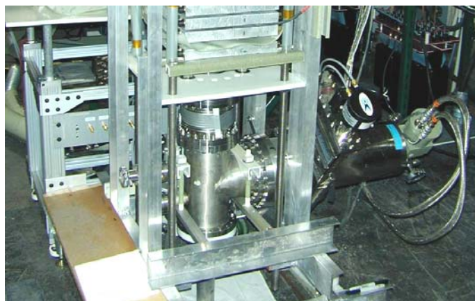
Figure 45. Cryopump, gate valve, and lower vacuum hardware
