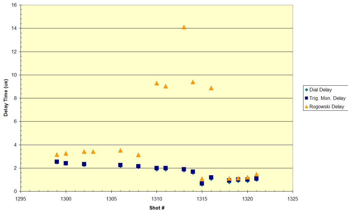
Figure B3. Delay data presented in Table B2 vs. shot number
