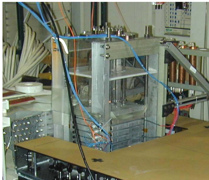
Figure 56. Blue fibers used for side-on fiber-optic array
