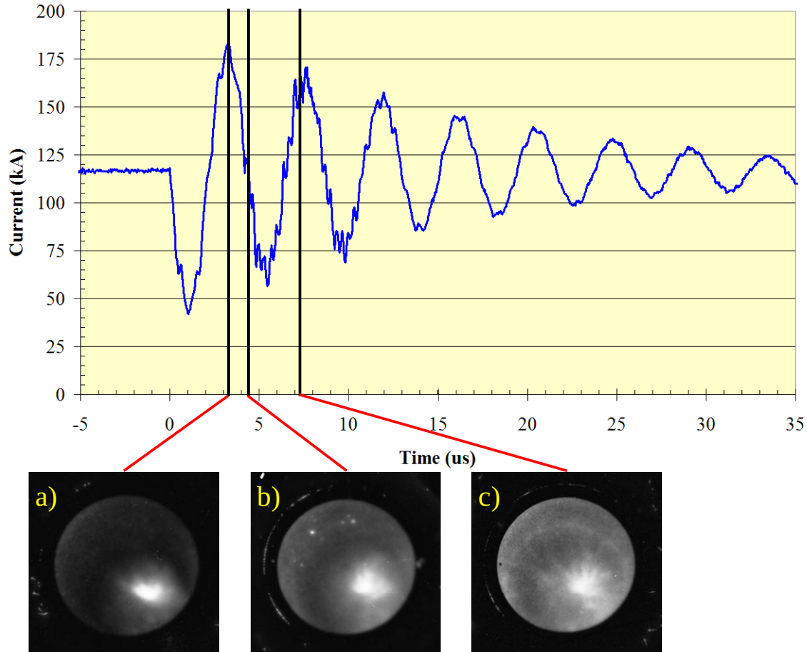
Figure 31. Theta coil current along with three MCP camera images
