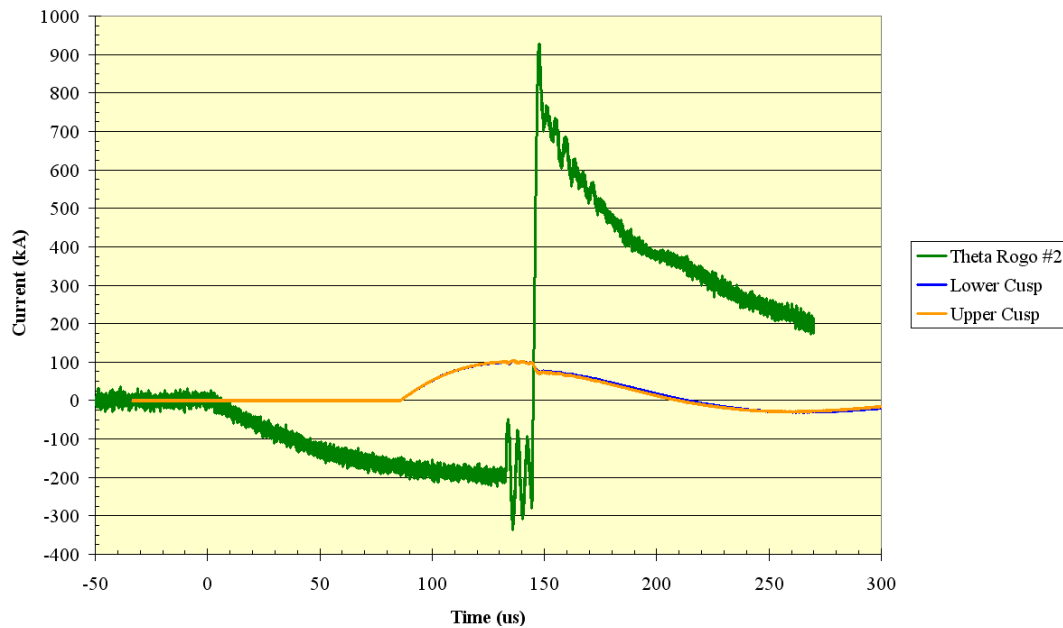
Figure 87. Theta and Cusp coil current waveforms from Test #7 in Figure 86
