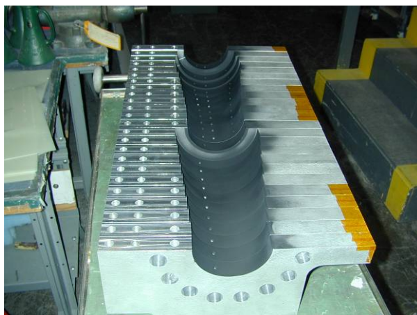
Figure 107. (a) Modified Cusp and Theta coil segments; (b) close-up view of tapped holes added to several coil-segment halves
