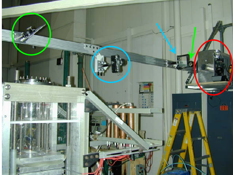
Figure 57. UNR end-on photography and fiber-probe diagnostics
