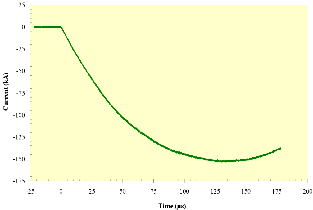
Figure 83. Bias current waveform from test #4, 3 Mar 2008
