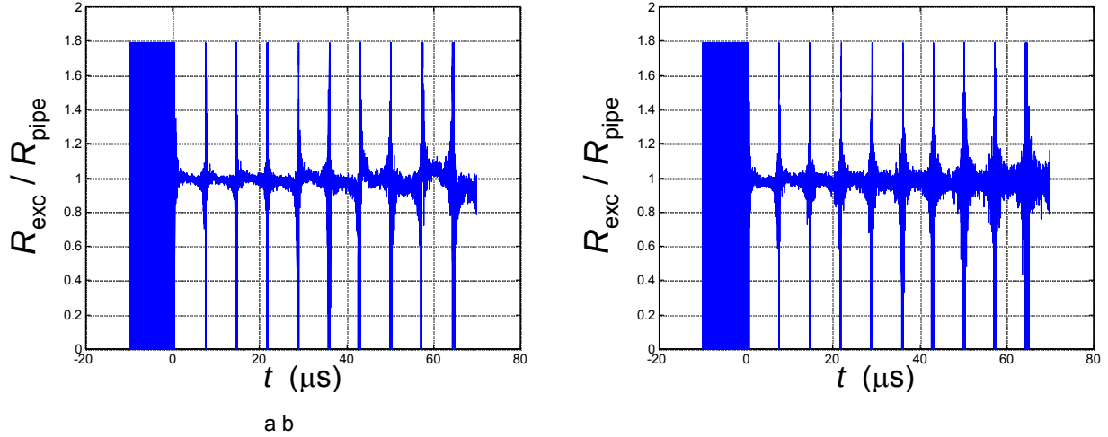
Figure 82. Excluded flux radius to pipe radius for single-cable setup using (a) short time-scale integrators; (b) long time-scale integrators
