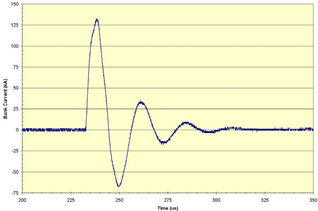
Figure 21. Discharge-current waveform for Crowbar Auxiliary bank
