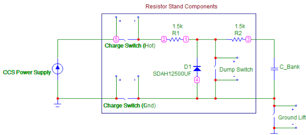
Figure 3. Basic charging and dumping circuit for both PI and Bias banks
