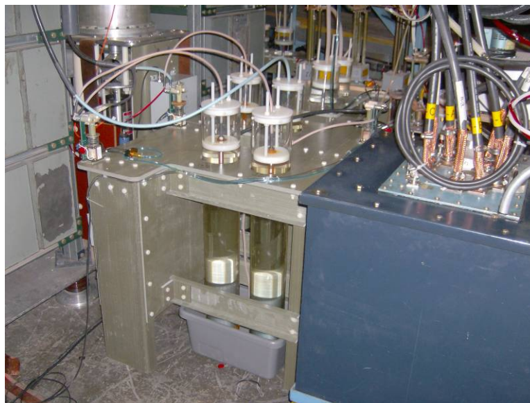
Figure 99. Two resistor stands for Guide/Mirror bank placed side by side
