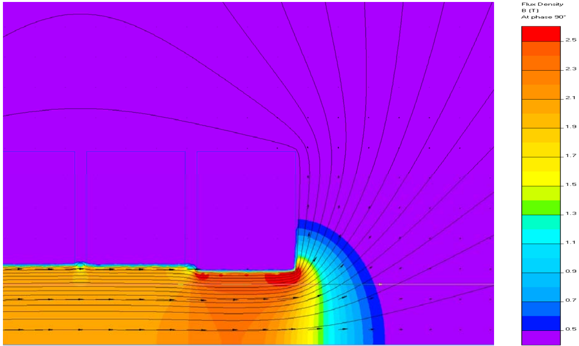
Figure A3. Magnetic flux density around field-coil segments
