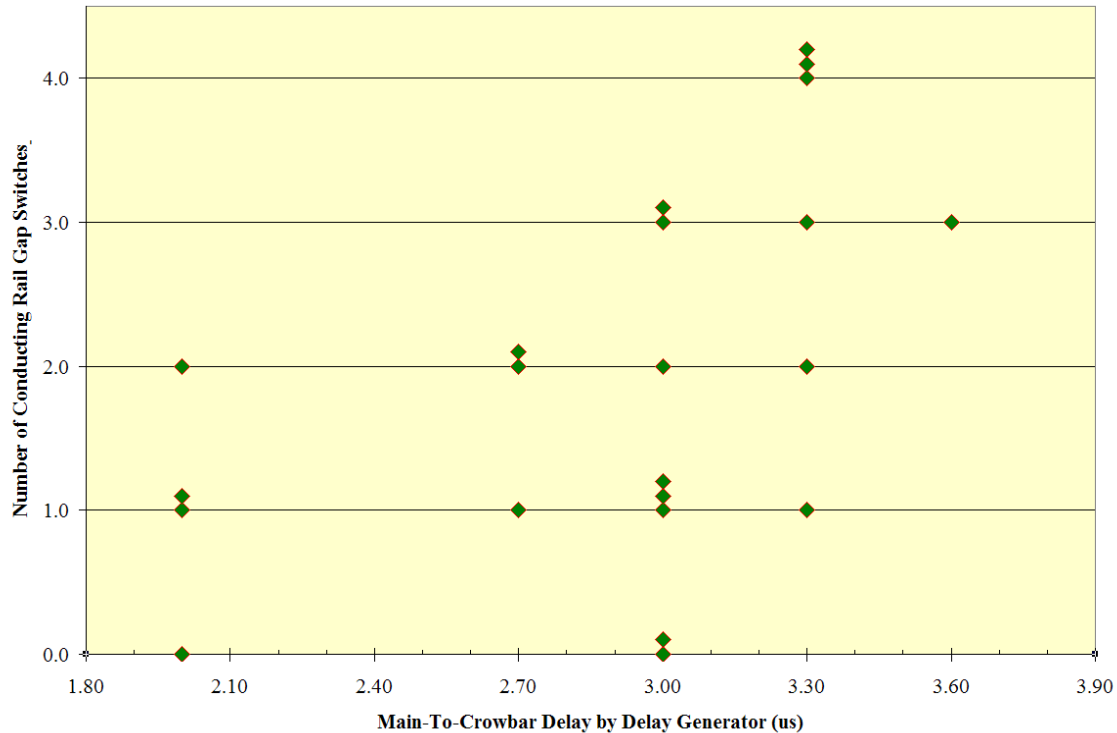
Figure B12. Number of rail gaps conducting in Crowbar switch vs. Main-to-Crowbar trigger delay The peak of the Main bank current is at approximately 3.3 \mu s. In Table B6 the delay values shown in green are comparable to the jitters observed with the first Crowbar switch. Delay values that are negative are shown in red in the table and indicate a pre-fire of that particular rail-gap switch.
