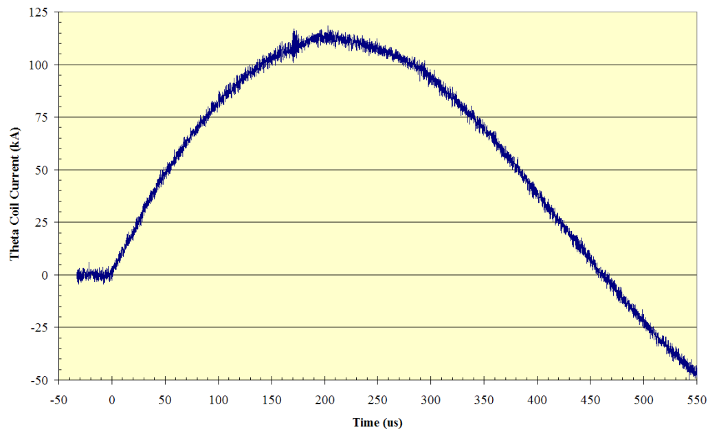
Figure 29. Theta coil current (averaged) for a Bias-only shot, two-module Bias bank
