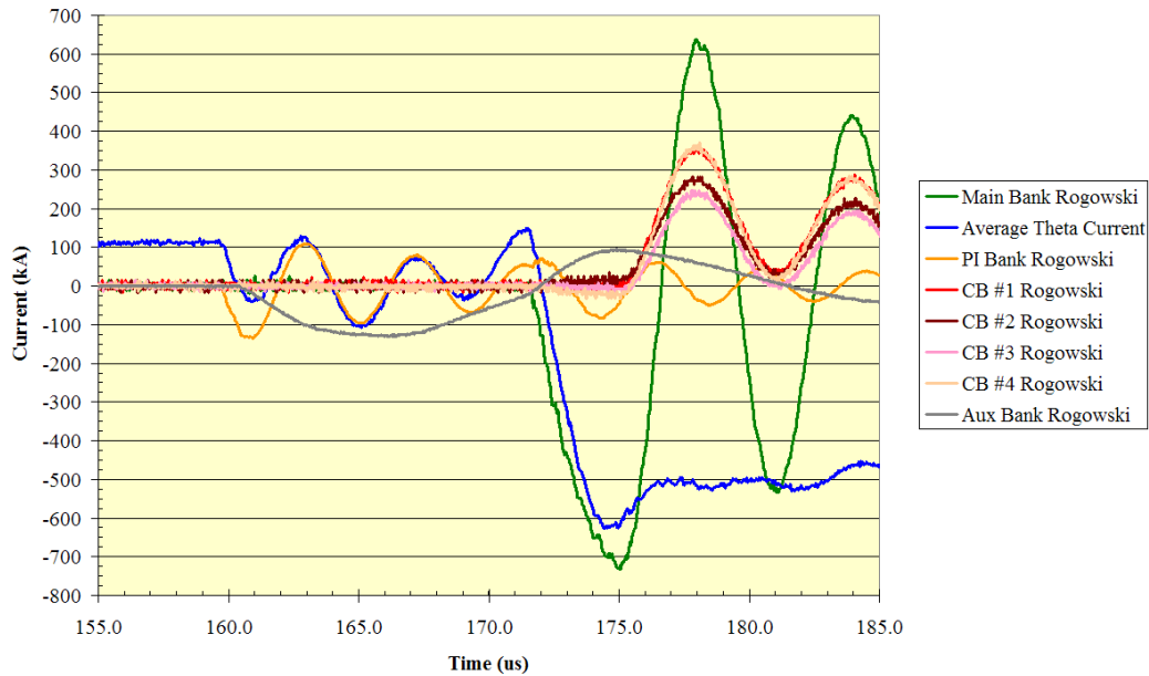
Figure 23. Bank-current waveforms, shot in which Auxiliary bank pre-fired
