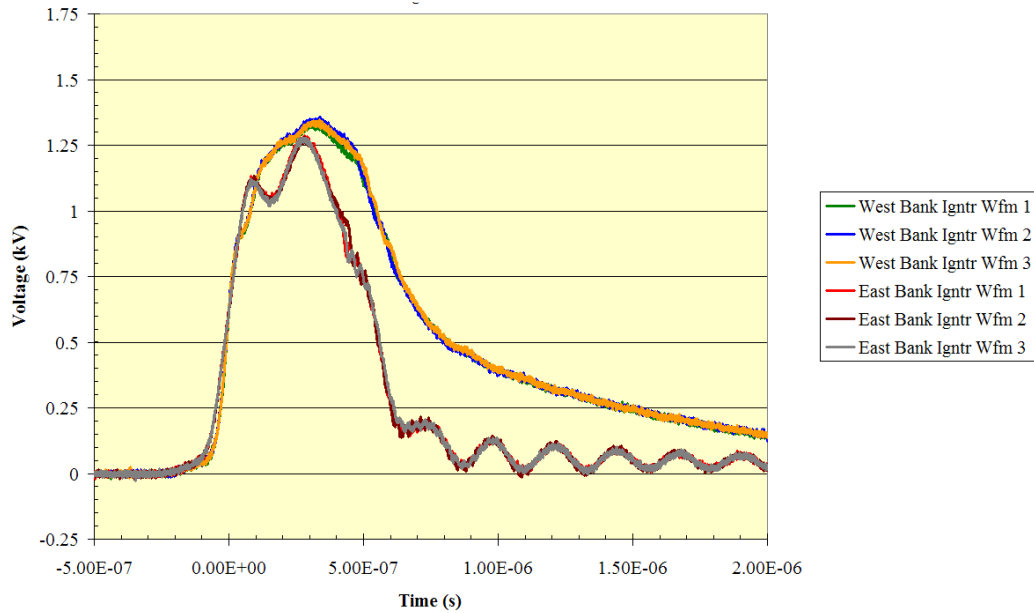
Figure 28. Three trigger pulses from each secondary of ignitron trigger transformer The pulses are not identical in amplitude or in pulse width, but their rise times are virtually the same, so the igniters of both ignitrons should spark nearly simultaneously.
