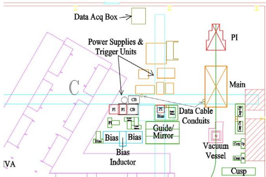
Figure 60. Test area showing placement of shielded enclosure and data-cable conduits
