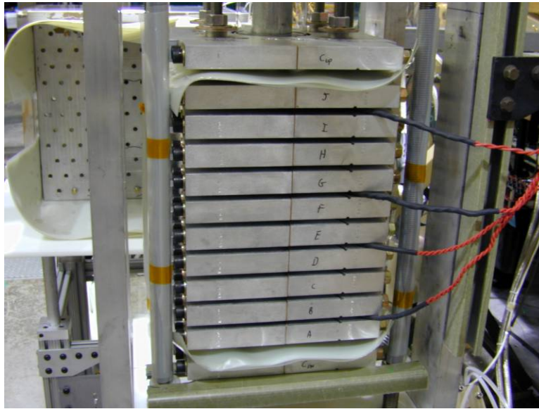
Figure 49. Completed Theta and Cusp coil assembly on vertical stand
