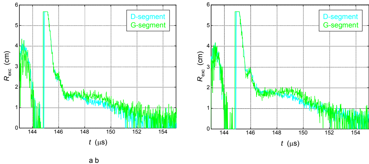
Figure 89. FRC excluded flux radius vs. time calculated, (a) Test #6; (b) Test #7
