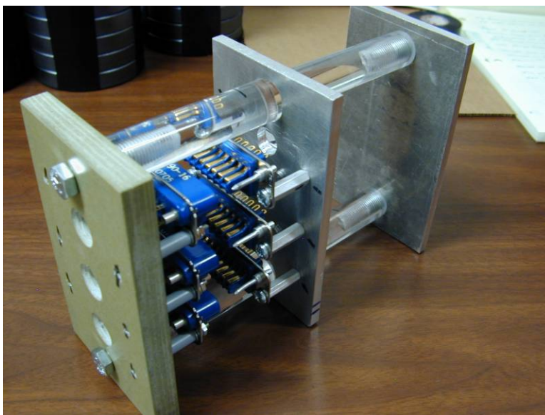
Figure 76. Pneumatically actuated set of contacts
