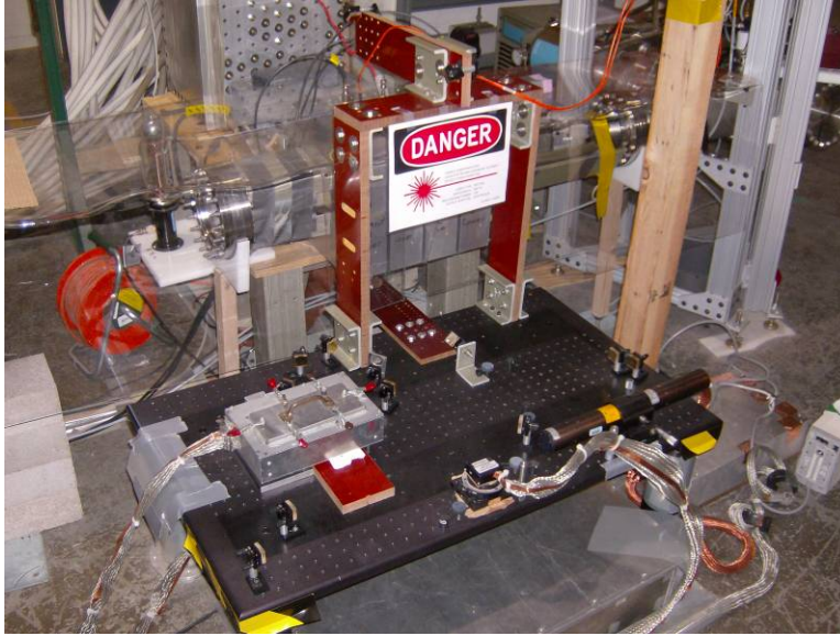
Figure 18. Single-chord interferometer in position in front of FRCHX Theta coil
