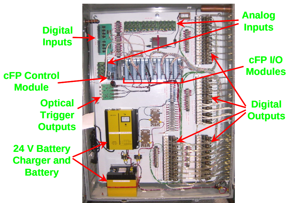
Figure 66. Controller components in Hammond enclosure
