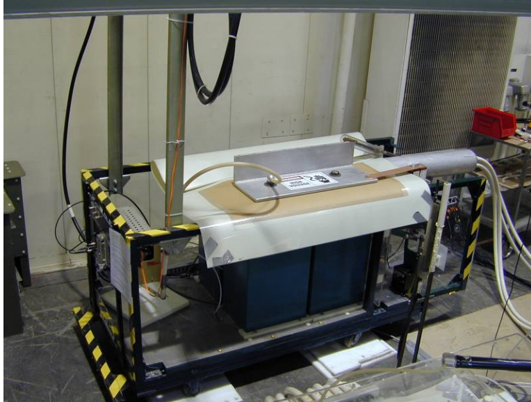
Figure 20. Completed Crowbar Auxiliary bank in place behind Main and PI banks
