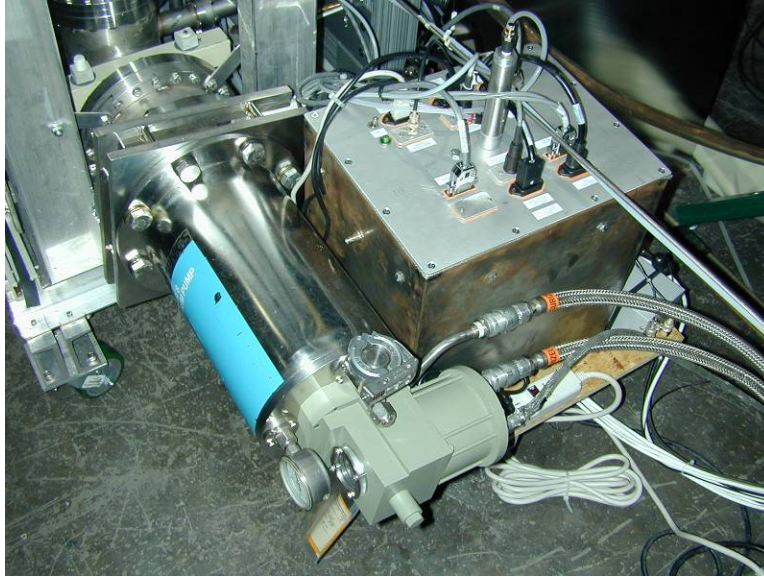
Figure 77. Gauge controller disconnect box on vacuum and field-coil stand
