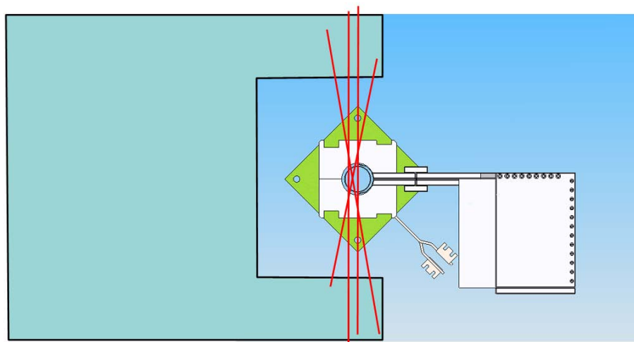
Figure 15. Placement of four-chord interferometer around FRCHX coils
