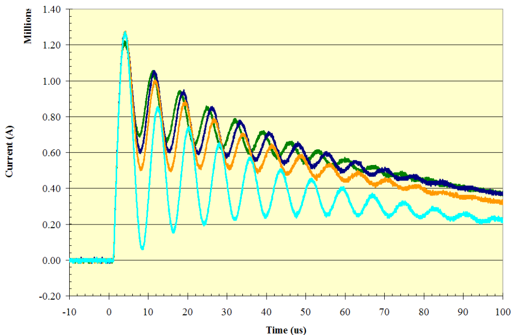
Figure B2. Overlay of load-current waveforms from shots 37, 38, 39 and 40
