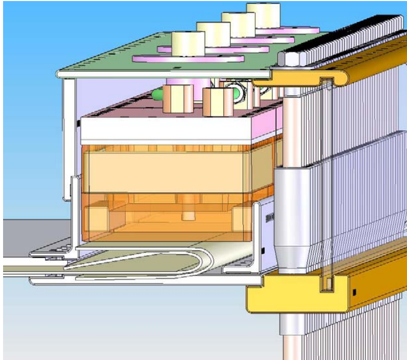
Figure C1. Basic Crowbar switch design
