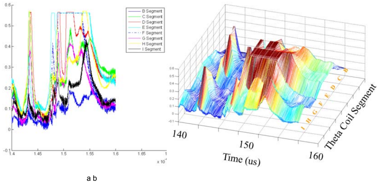
Figure 91. Side-on fiber-optic-array data: (a) signal intensity vs. time; (b) surface plot Though a number of the waveforms was clipped, the primary feature to look for is whether or not some of the signals decreased to zero while others, particularly those at either end of the Theta coil, persisted for a longer period of time or trailed off in a sequential fashion. What is observed, however, is that there was no particular grouping of channels that had signals that persisted for
