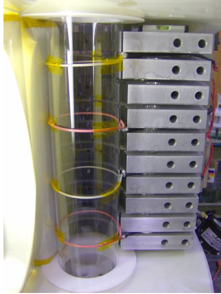
Figure 47. Cylindrical Theta coil, with six-segment uniform region in the middle bounded by two-segment mirrors top and bottom
