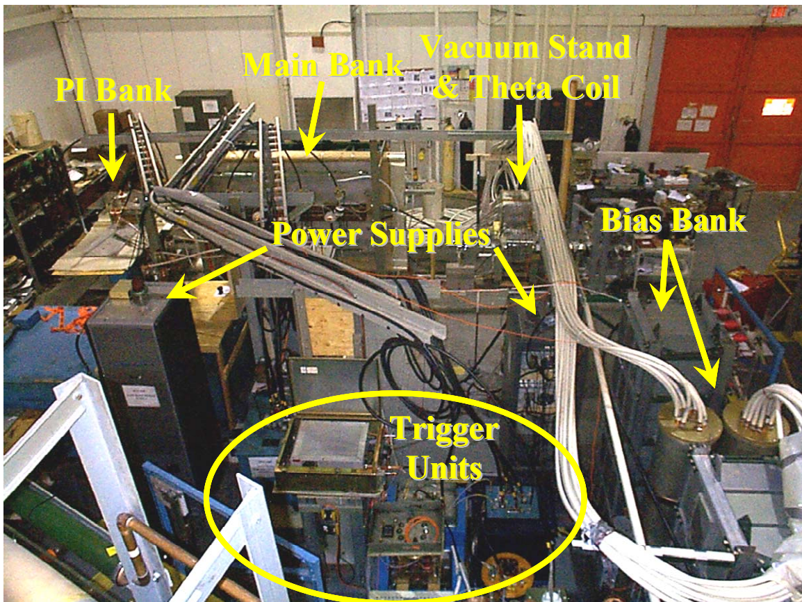
Figure 1. View from Shiva C-arm of early FRCHX experimental setup
