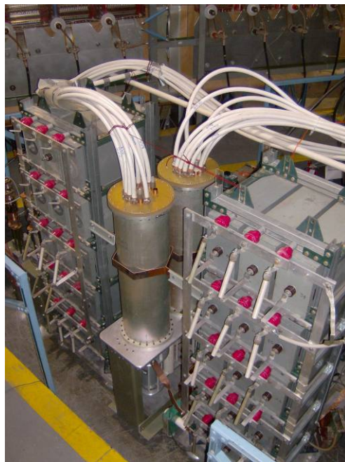
Figure 2. Bias bank just after its assembly was completed
