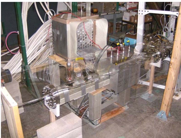
Figure 11. Temporary Theta coil, support stand, and vacuum system
