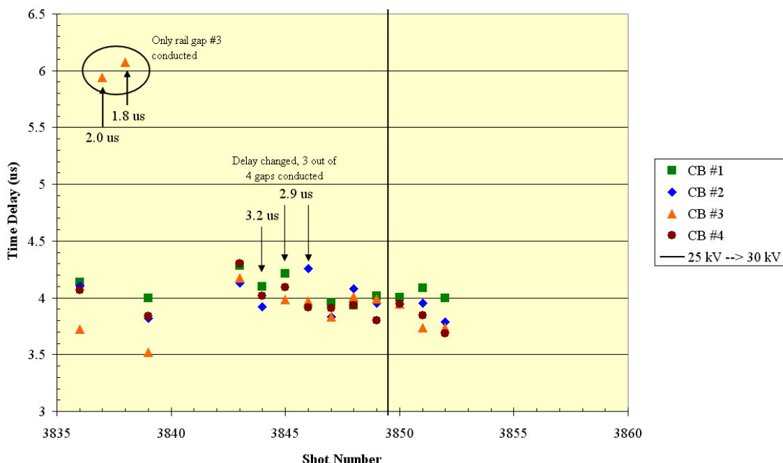
Figure B10. Enlarged view of data in Figure B8
