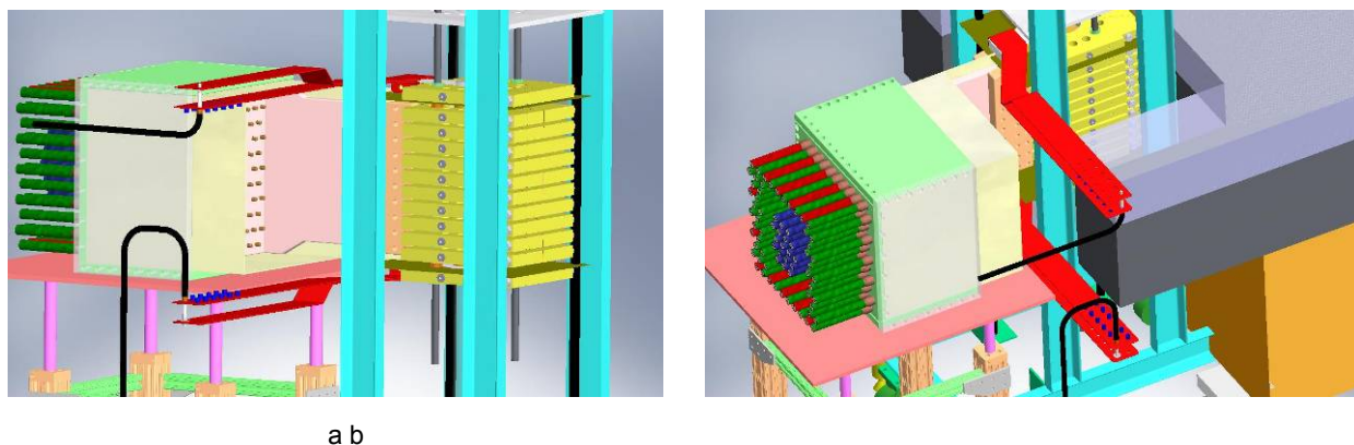
Figure 37. (a) and (b) Cusp coil bus plates
