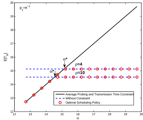
Fig. 4. E[T_N] of network versus average probing and transmission time constraint of \alpha
