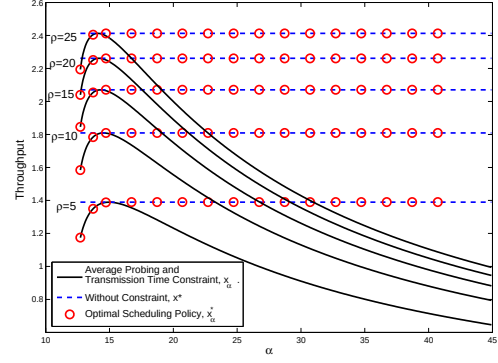
Fig. 3. Maximal throughput for different values of \alpha at different \rho
