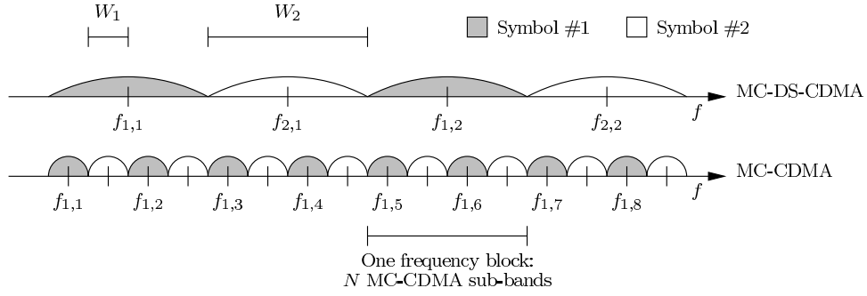
Fig. 3. Spectra of the MC-DS-CDMA and MC-CDMA signals. In this example, M = 2 parallel data symbols are each repeated across R_1 = 8 and R_2 = 2 sub-carriers in MC-CDMA and MC-DS-CDMA, respectively, where N = 4 is the processing gain in each MC-DS-CDMA sub-band. We assume the coherence bandwidth of the channel, (\Delta f)_c , is equal to W_2 .
