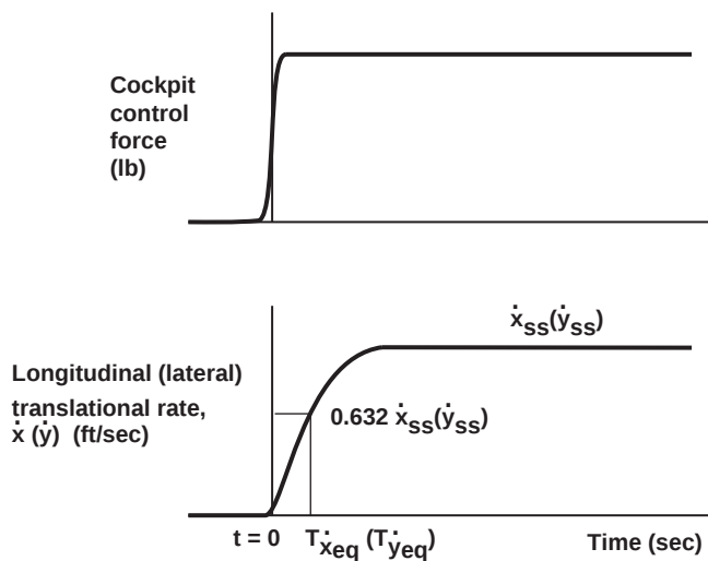
a) Definition of equivalent rise time, T_{\dot{x}eq} (T_{\dot{y}eq})
