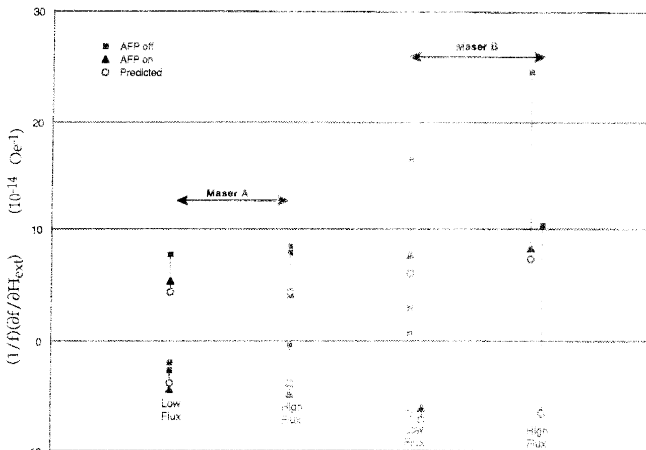
Fig. 5. Effect of State Selection on Magnetic Sensitivity
