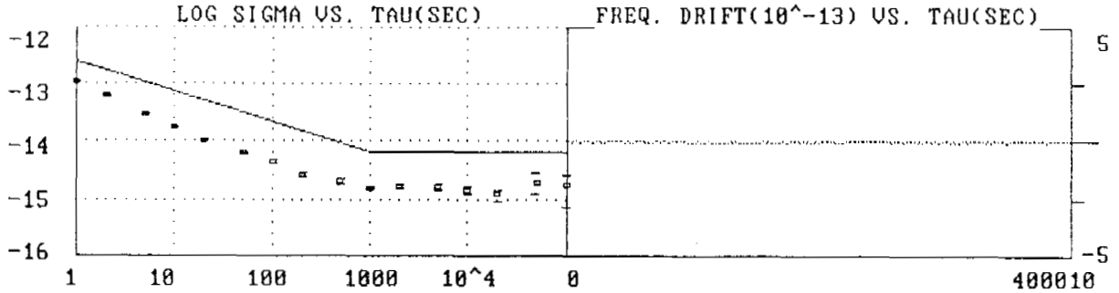
Figure 4. STSC measurement of maser stability.
