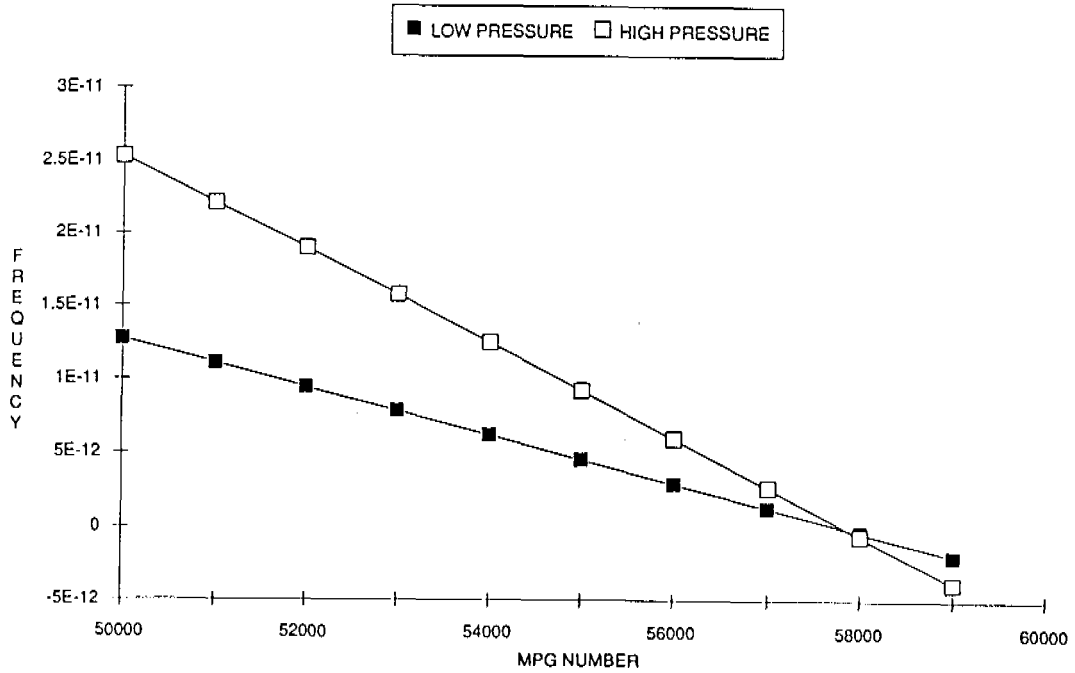
Figure 1. Spin-exchange tuning a STSC hydrogen maser equipped with a cavity frequency switching servo.
