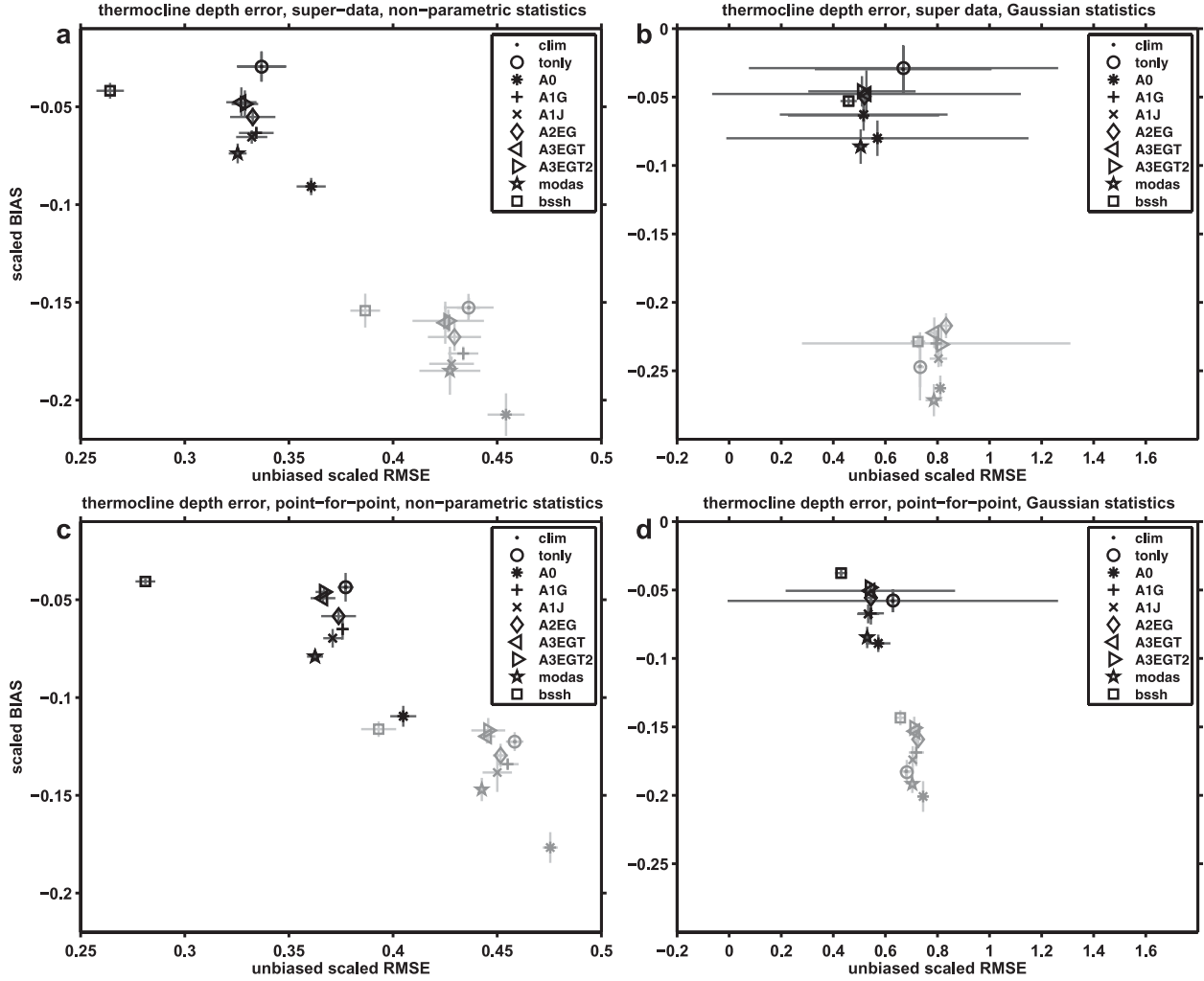
FIG. 6. (a) The superdata and nonparametric statistics summary diagram of \text{RMSE}_{\text{unbiased}}^{\text{bw}} ( x axis) and \text{MB}^{\text{bw}} ( y axis) for \text{TD}_{\Delta} (black and 75% gray error bars) and \text{TD}_{\nabla} (50% and 25% gray error bars) for the 10 synthetics denoted by the symbols in the legend as described in Table 1. (b) The superdata and Gaussian statistics summary diagram of \text{RMSE}_{\text{unbiased}}^{\text{bw}} ( x axis) and \text{MB}' ( y axis) for \text{TD}_{\Delta} (black and 75% gray error bars) and \text{TD}_{\nabla} (50% and 25% gray error bars). (c) The point-for-point data and nonparametric statistics summary diagram of \text{RMSE}_{\text{unbiased}}^{\text{bw}} ( x axis) and \text{MB}^{\text{bw}} ( y axis) for \text{TD}_{\Delta} (black and 75% gray error bars) and \text{TD}_{\nabla} (50% and 25% gray error bars). (d) The point-for-point data and Gaussian statistics summary diagram of \text{RMSE}_{\text{unbiased}}^{\text{bw}} ( x axis) and \text{MB}' ( y axis) for \text{TD}_{\Delta} (black and 75% gray error bars) and \text{TD}_{\nabla} (50% and 25% gray error bars). The error bars represent a 100 independent draw bootstrap standard error estimate.
