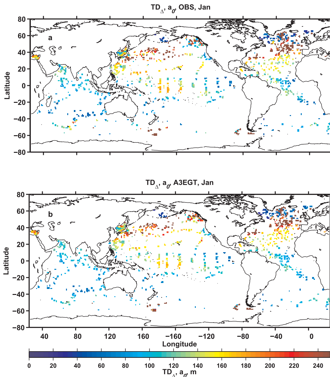
FIG. 4. The fit parameter a_0 (superdata mean; in m) for the (a) observed and (b) A3EGT synthetic TD _{\Delta} estimate for the global ocean for a 60-day analysis window starting 1 Jan for the years 2001–03.
