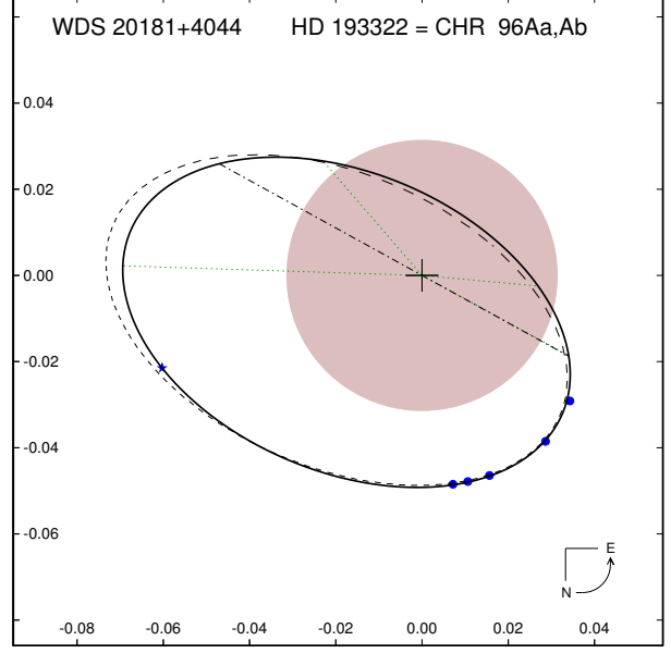
Fig. 2. Orbit of HD 193322. Symbols are as in the earlier figure, with the star now indicating a CHARA Array measure. The dashed ellipse here represents the orbit of Hartkopf et al. (1993).
