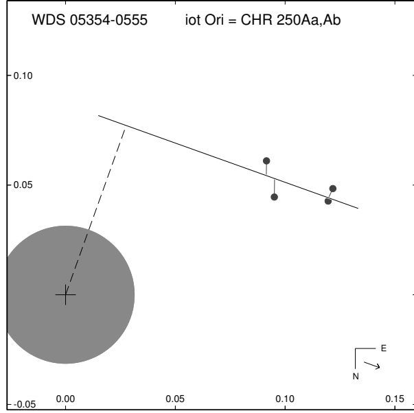
Fig. 3. The \iota Ori speckle pair. This rectilinear fit made to speckle measures dating from 1994.7–2006.2 predicts the pair reached a closest apparent separation of 0''.076 in 1966. We may of course be viewing a small arc of an orbit instead, but the period of such an orbit would be much longer than 40 years.
