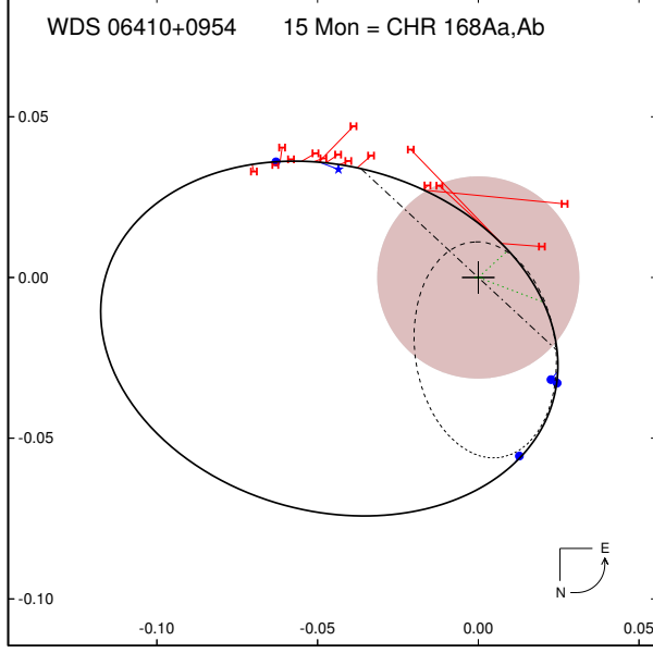
Fig. 1. Orbit of 15 Mon. Speckle measures are shown as filled circles, an NPOI measure as a filled star; “H” symbols are HST FGS measures. “O – C” lines connect data points to their predicted locations on the orbit. The large shaded circle represents the Rayleigh resolution limit of a 4 m telescope. Dotted lines from the origin denote predicted positions of two unresolved measures. The dot-dash line is the line of nodes; the dashed ellipse is the orbit of Gies et al. (1993). Scales are in arcseconds.
