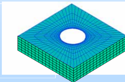
Open Hole Models
