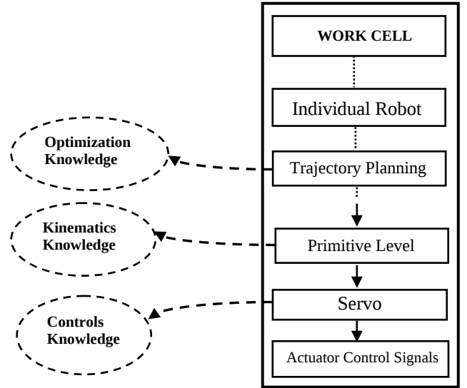
Figure 2: Various activities related to robotics domain
