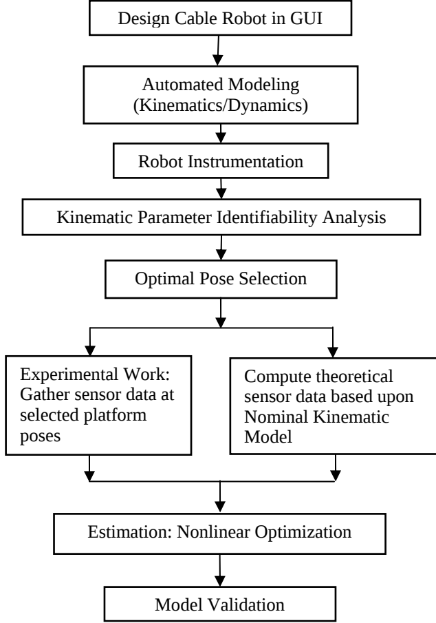
Figure 1: Cable robot calibration process
