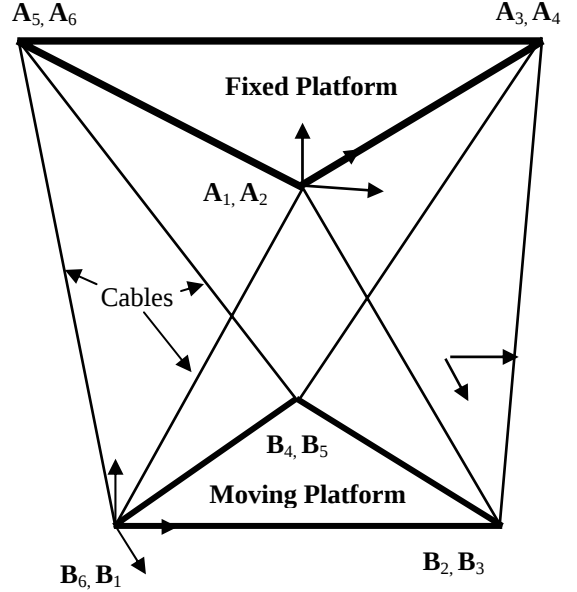
Figure 5: A Six DOF cable robot
