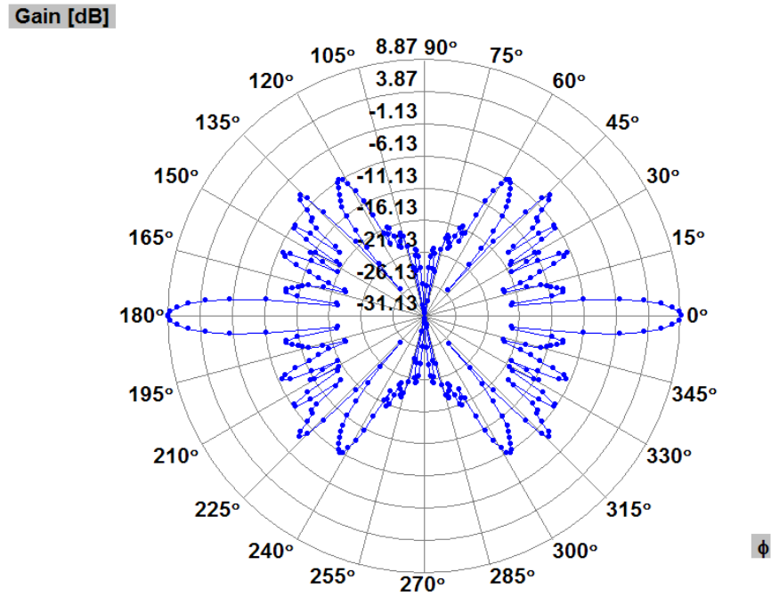
Figure 21. Azimuth Radiation Pattern for Fore/aft Antennas
