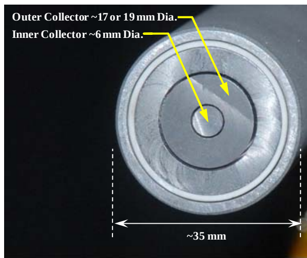
FIG. 2. Photograph of the AFRL nested Faraday probe shown in the 0.5-mm gap width configuration.
