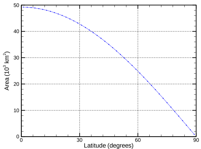
Figure 8. Area at the surface of the Earth of a 2^\circ \times 2^\circ rectangular box, as a function of latitude.
