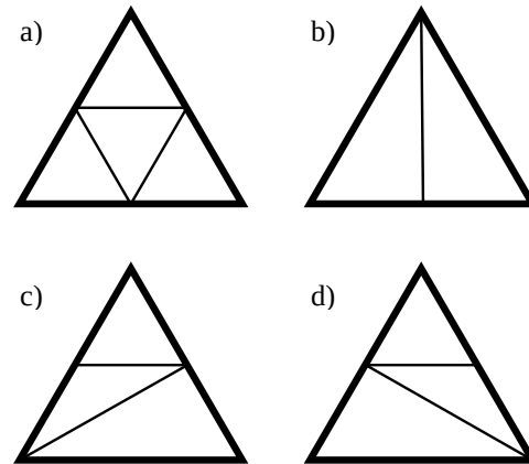
Figure 5. An illustration of some of the ways in which a triangle can be subdivided into smaller triangles. a) three new vertices, b) one new vertex, c and d) two new vertices.
