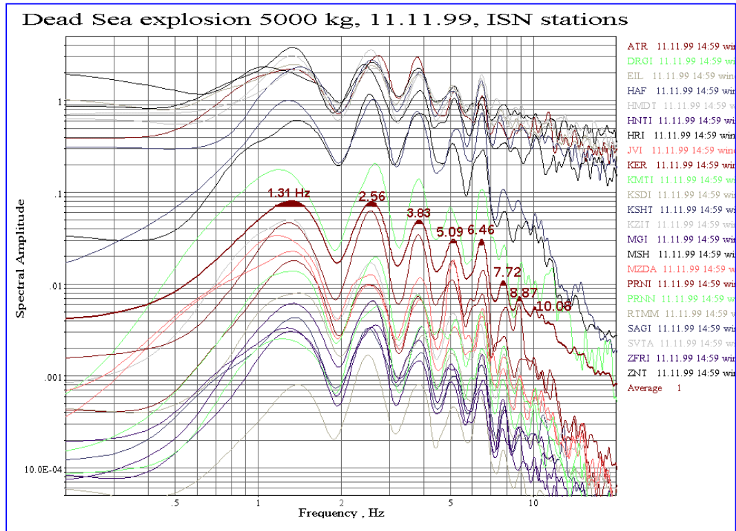
Fig. 7. Determination of the bubble frequency from smoothed averaged spectra of ISN seismograms.
