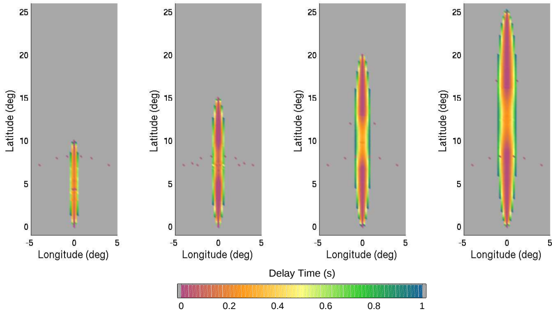
Figure 4: Delay time, minimized over depth, as a function of latitude and longitude for four source-receiver paths with epicentral distances of 10°, 15°, 20°, and 25° (left to right).
