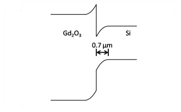
Fig. 35 A simple band structure model of the Gd2O3/Si heterojunction. The electric field created by the applied bias is limited to a region approximately 0.7 \mu\text{m} in length.
