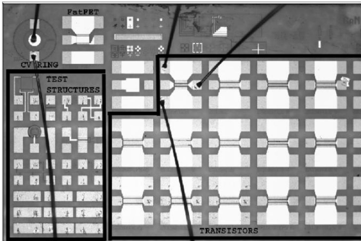
Figure 10. Devices deposited on an AlGaIn/GaN wafer. FATFETs were used in this research due to increased vulnerability to radiation.
