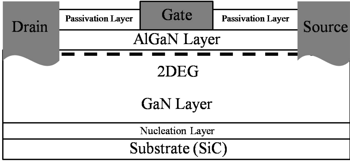
Figure 3. HFET's cross section showing formation of 2 DEG [8] at the AlGaN/GaN interface.
