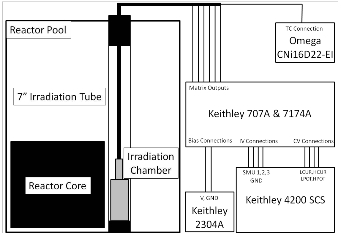
Figure 12. Test setup shows basic connections between the data acquisition system.
