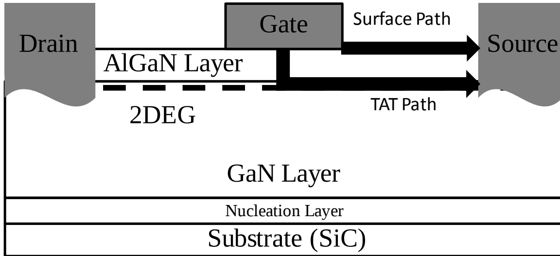
Figure 29. Proposed leakage current paths. The probability of carriers flowing through the path along the top of the AlGaN layer was increased due to irradiation induced oxygen complexing of the AlGaN layer.
