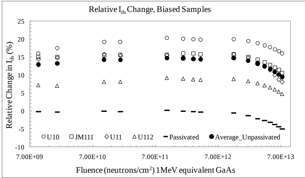
Figure 18. Relative current change in biased samples.
