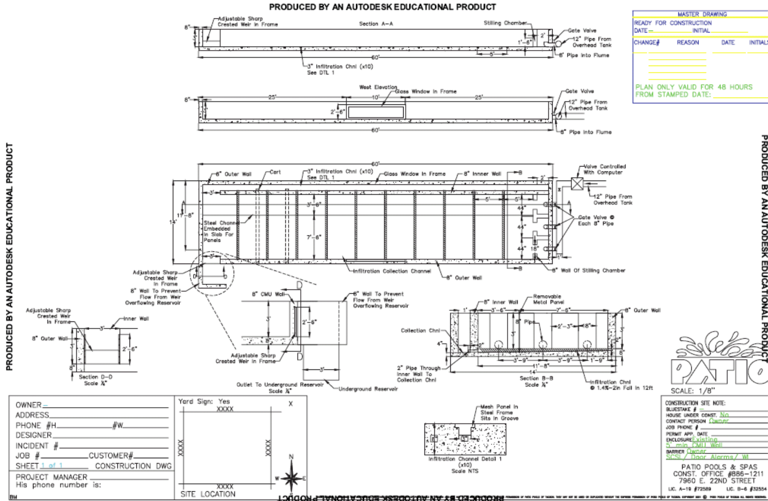
Fig.1 Upgraded new flume design - planform
